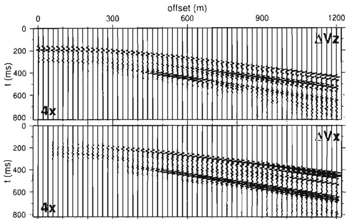
Figure 4: Difference AVO responses, obtained by subtracting traces calculated for 25% \text{CO}_2 saturation from those for 100% water saturation in a porous sandstone layer (Aldridge & Bartel, Sandia Natl. Labs).
