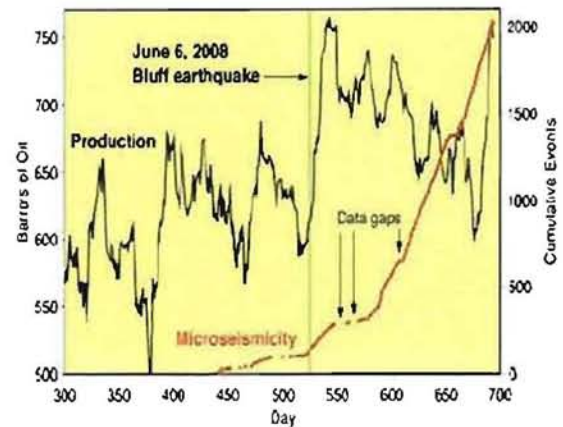
Correlation of increased oil production and reservoir seismicity following local earthquake.
