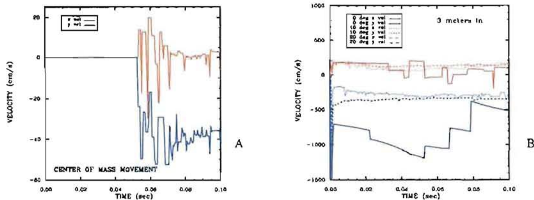
Figure 2. In panel A, we show the velocity at the center of the target for a 100 m diameter basalt sphere exposed to a 100 kt burst 70 m from the surface. The shock hits the center about 0.05 s after the burst and the y-axis velocity reaches 35 cm/s by 0.1 seconds. In panel B, we show the expansion velocity of material near the surface of the basalt sphere. The expansion velocities can be as high as 10 m/s (1000 cm/s) and is concentrated in a cone with a half-angle of 30 degrees
