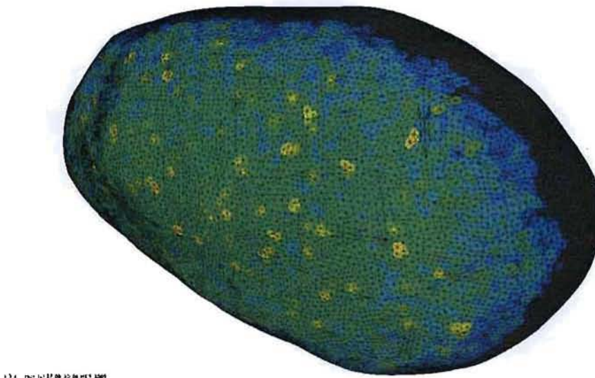
Figure 3. Example of neutron irradiation of an Itokawa shape asteroid model by a 100-kt device with a Trinity test neutron energy spectrum. The source is to the left of the page. The yellow spots are the result of Monte-Carlo noise.
