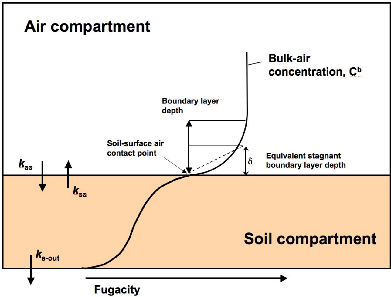
Figure 4. An illustration of the role of mass transfer coefficients in establishing mass balance in a two-compartment system consisting of soil and air.
