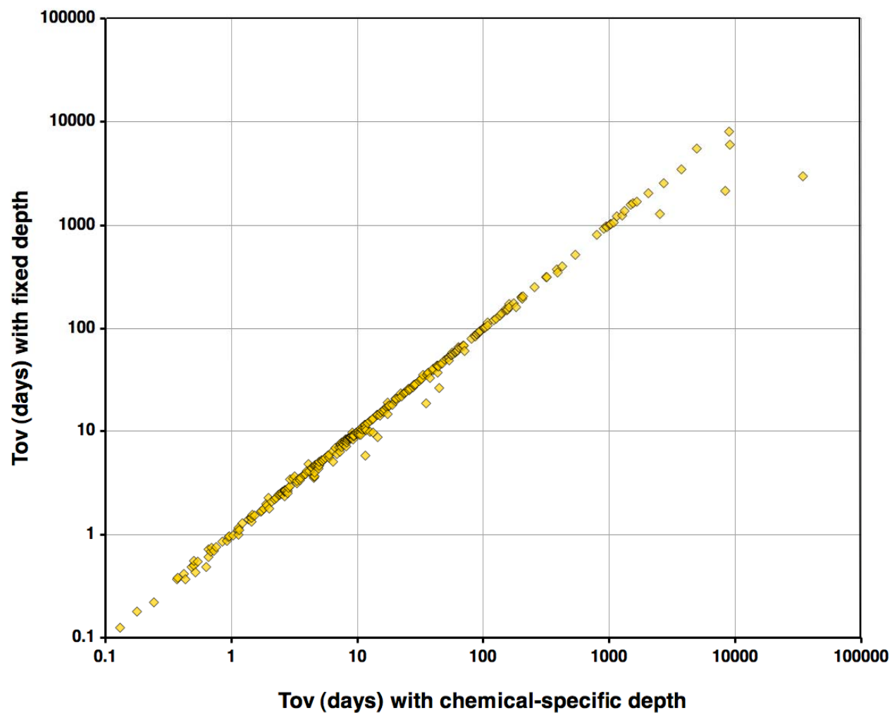
Figure 5. An illustration of how the model output overall persistence (Tov in days) varies among 300 chemicals between a two-compartment model using a fixed depth in the range of 0.1 to 0.15 m and the same model using a chemical-specific depth, which is ds = z^* .
