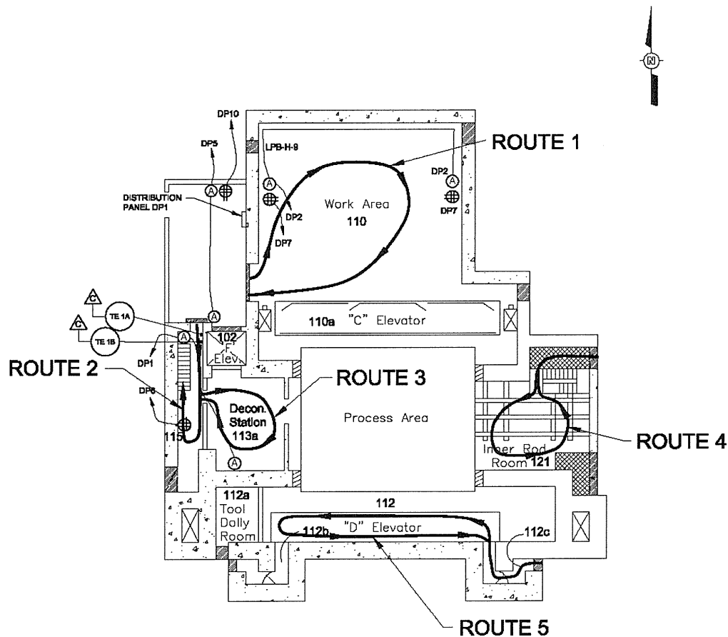
Figure 2-4. General Plan of 105-H Safe Storage Enclosure at Ground Level.
