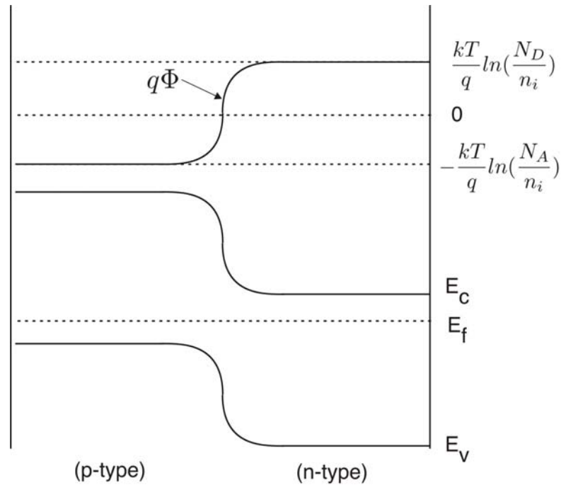
Figure 2.2. Neutral Contacts.
