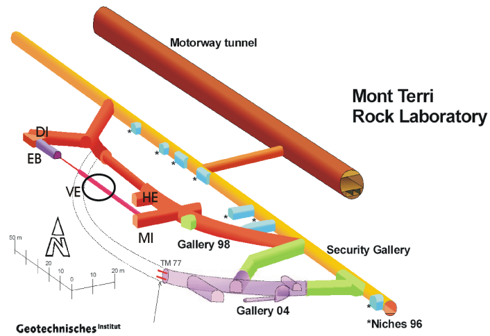
Fig. 1. Layout of Mont Terri underground research laboratory and location of the Ventilation Experiment, VE (Fernández et al. 2006).
