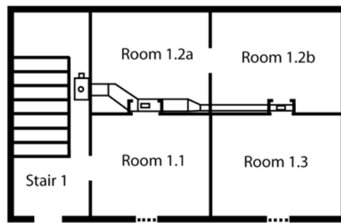
Figure 3: First floor plan view. The intake for the recirculating fan unit is in the stairwell. Outlets are in Rooms 1.2a, 1.2b, and two rooms on the second floor.
