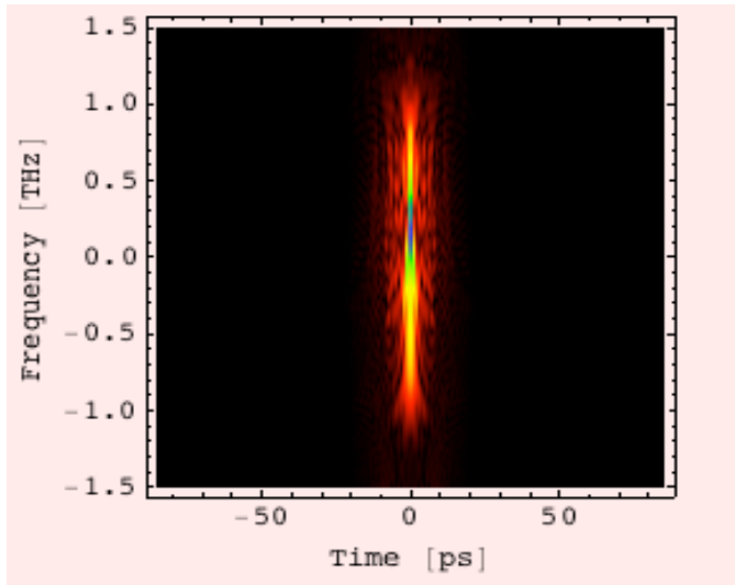
Fig. 9. High resolution experimental FROG trace of compressed 800nJ pulses with B=1.4
