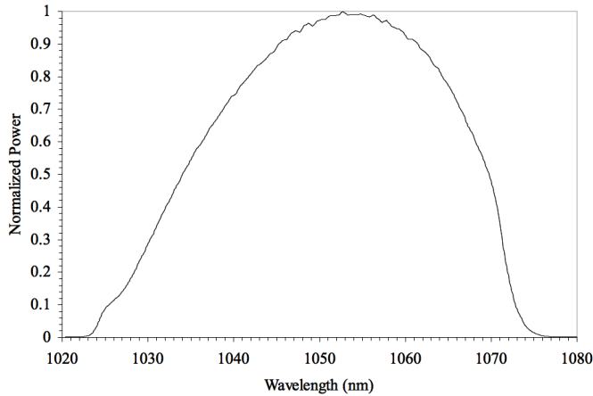
Fig. 3. Spectrum from mode locked oscillator taken with an ANDO Optical Spectrum Analyzer with a resolution bandwidth of 0.1 nm.
