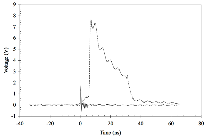
Fig. 4. Data from pre-pulse contrast measurement at input to the ASE pulse cleaner. The solid line is the attenuated pulse and the dashed line is the unattenuated pulse. The ASE pedestal is clearly visible in the unattenuated pulse as a foot prior to the rapidly rising main edge of the unattenuated pulse.
