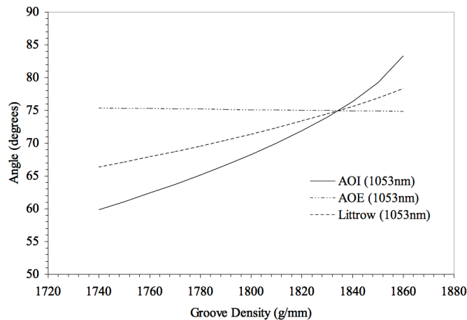
Fig. 13. Angle of incidence (AOI), output angle (AOE) and Littrow angle at 1053nm as a function of groove density for a Treacy compressor with the TOD/GDD ratio needed to construct pulse twacker A.
