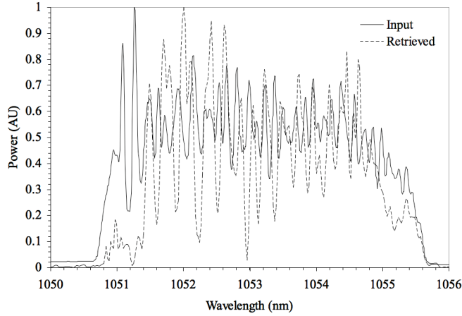
Fig. 12. Comparison of the measured and retrieved pulse spectrum for the 58 \mu\text{J} pulses.
