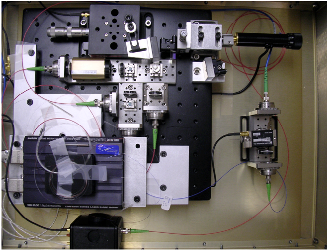
Fig. 2. (a) Schematic of the fiber mode locked oscillator (b) picture of the assembled oscillator viewed from the top
