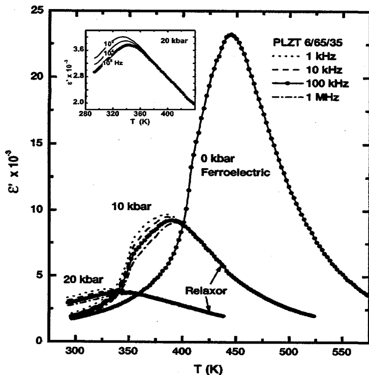
Fig. 1. Pressure-induced FE-R crossover in PLZT 6/65/35.
