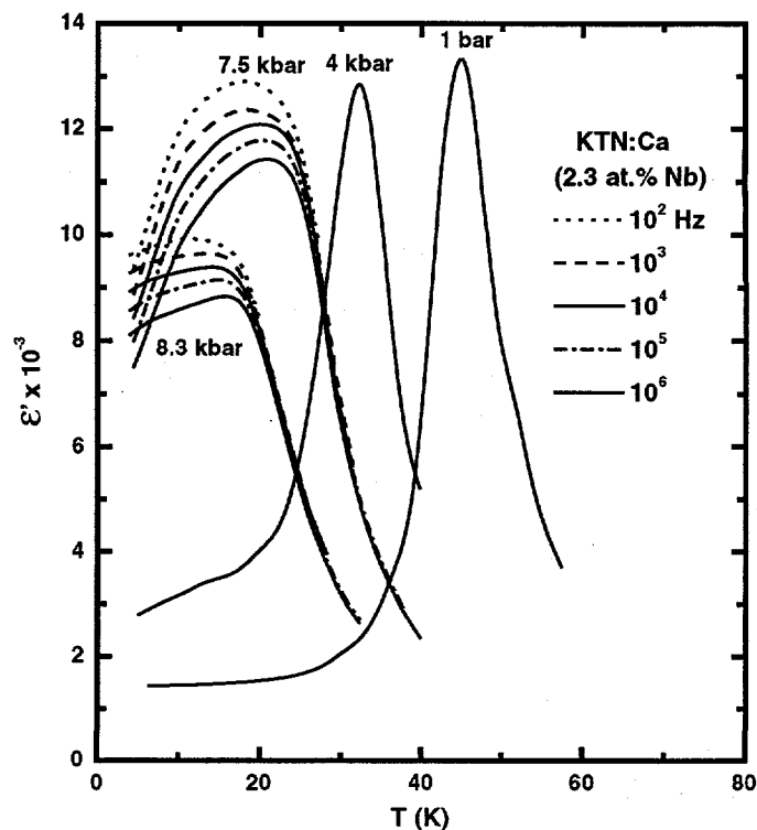
Fig. 2. Pressure-induced FE-R crossover in KTN.
