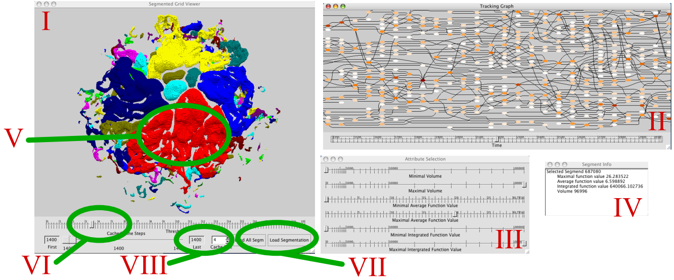
Figure 2. User interface of our framework: (I) 3D display of the segmentation including a slider to select the fuel consumption threshold (VI), the interface to determine the number of in-memory time steps (VIII), and the button to load the geometry (VII); (II) Interactive display of the tracking graph. Selecting node in either the 3D viewer or the graph display causes the corresponding cell to be highlighted (v) and its attribute information to be displayed in the info window (IV). The last window (III) provides the ability to sub-select segments based on attribute values.
