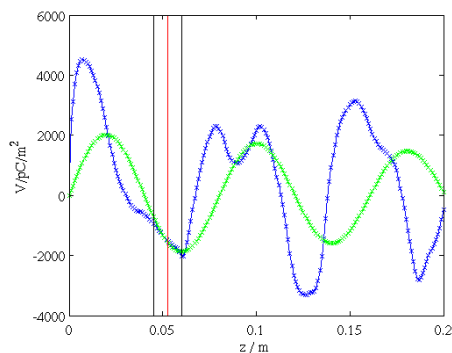
Figure 2: Measured time-domain wake (blue), compared with the simulated frequency domain wake (green), with the position of the 2nd bunch marked (red), \pm 5\sigma (black).
