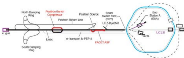
Figure 1: Schematic of the planned layout of FACET.
