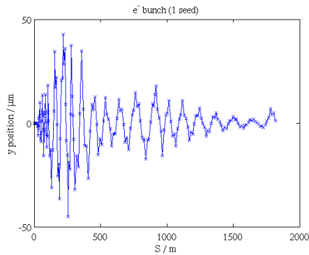
Figure 4: Example of 1 seed of tracking for the electron bunch, showing the orbit excited by coupling from the positron wake.
