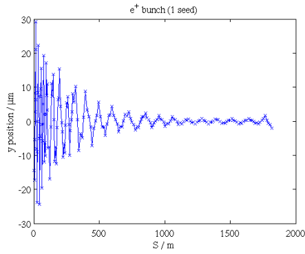
Figure 3: Example of 1 seed of tracking for the positron bunch, showing the orbit due to the off-centre initial bunch.
