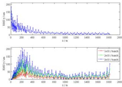
Figure 5: RMS jitter in the y plane for the e^+ bunch (upper plot), and the e^- bunch for a series of e^+ charges.
