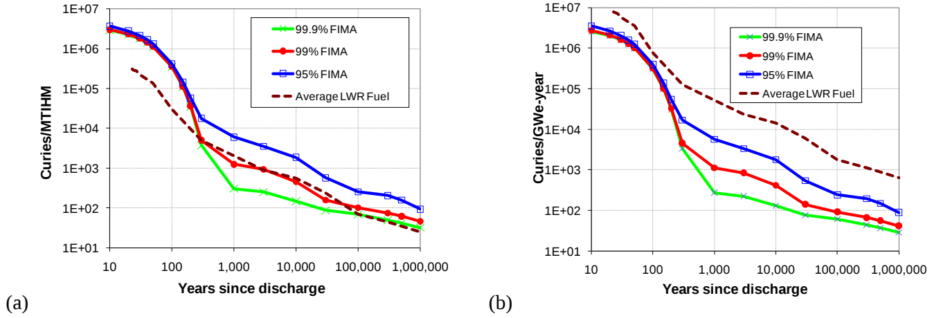
Figure 1. Activity of deep-burn fission waste compared to average spent LWR fuel
