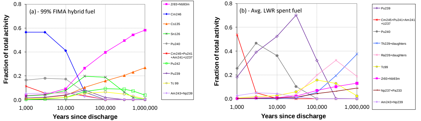
Figure 2. Fractional contribution of individual nuclides and decay chains to the total activity of (a) 99% FIMA hybrid fuel and (b) average LWR spent fuel for the period 1000 to 1,000,000 years post discharge. Figures include all nuclides or chains contributing > 5% to the total activity at any time during these periods.
