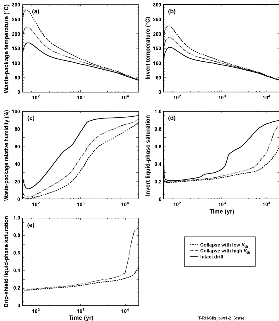
Fig. 9. Thermal-hydrologic (TH) conditions are plotted for a location close to the center of the repository for the low-probability-seismic drift-collapse scenario, and for the low and high rubble-thermal-conductivity K_{th} cases. The plotted TH parameters are (a) waste-package temperature, (b) invert temperature, (c) waste-package relative humidity, (d) invert liquid-phase saturation, and (e) drip-shield liquid-phase saturation.
