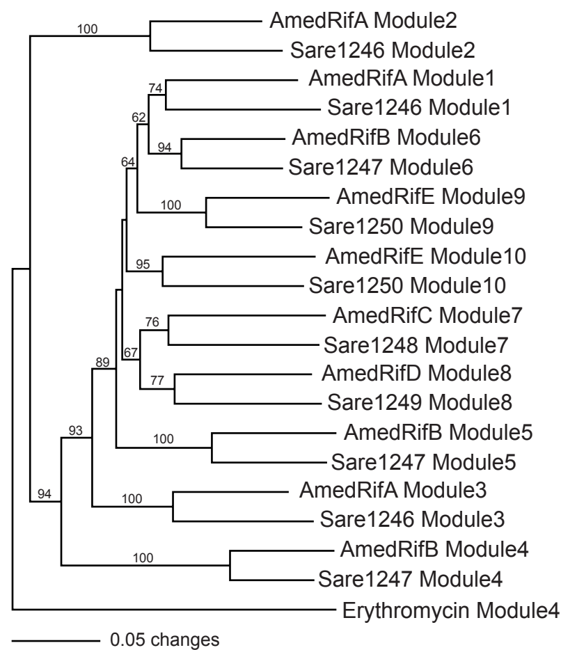
Supplementary Figure 1. Polyketide synthase phylogeny. Neighbor-joining distance tree constructed using the aligned amino acid sequences of the rif KS domains from A. mediterranei and S. arenicola . Bootstrap values (in percent) calculated from 1000 re-samplings are shown at their respective nodes for values greater than or equal to 60%. The KS domain from module 4 of the erythromycin biosynthetic pathway ( Saccharopolyspora erythraea ) was used to position the root.
