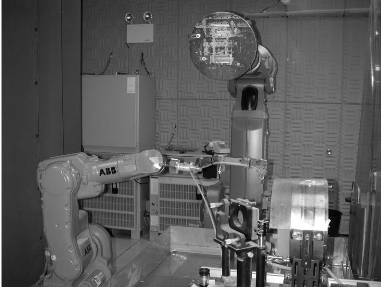
Figure 8 LLNL laser peening treatment area. Six-axis robotics were used for maneuvering coupons for treatment. Note the use of sound absorbing material on the back walls. The laser peening treatment generates >130 dB sound pulses as the shockwave propagates through the material.
