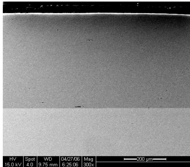
Figure 16 SEM image of the 316L laser peened coupon with no cathodic charging.
