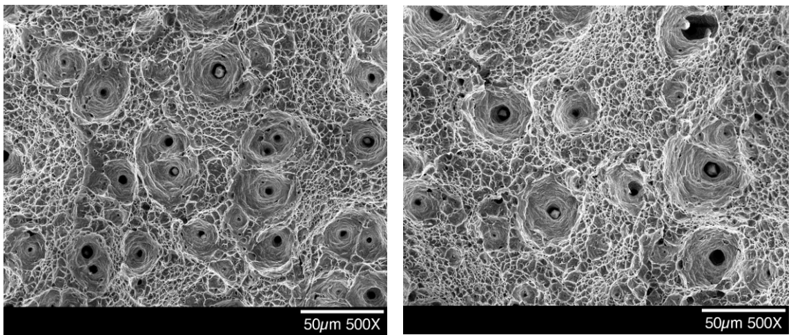
Figure 36 Left - As-received 21-6-9.
