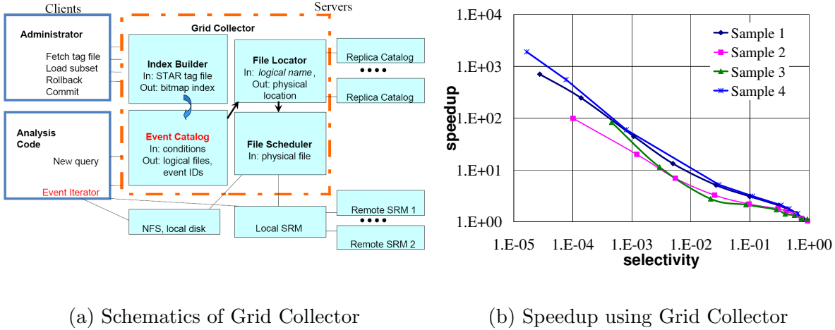
Figure 5: Using Grid Collector can significantly speed up analysis of STAR data (Timing measurements collected on a cluster with 2.8 GHz Intel Xeon processors [32, 42]).
