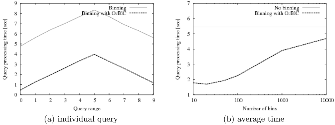
Figure 4: Time needed to process range queries using indexes with and without Order-preserving Bin-based Clustering (OrBiC) (Timing measurements collected on a 2.8 GHz Pentium 4 [40]).
