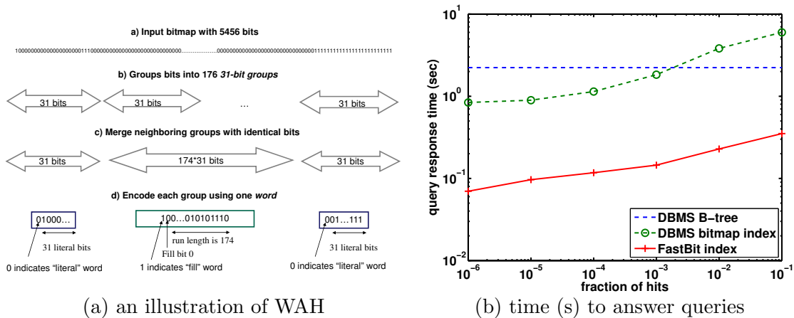
Figure 2: The effects of compression on query response time. The faster WAH compression used in FastBit reduces the query response time by an order of magnitude (Timing measurements collected with a 400 MHz UltraSPARC II CPU [36, 29]).
