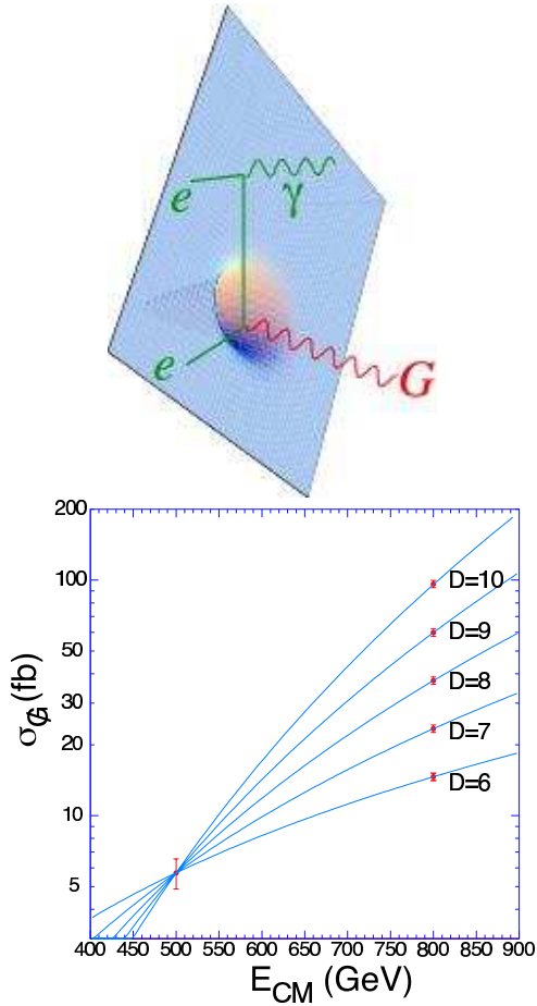
Figure 14. Top: Emission of a graviton into the hidden dimensions. Bottom: The energy dependence of the rates for various number of dimensions. 7
