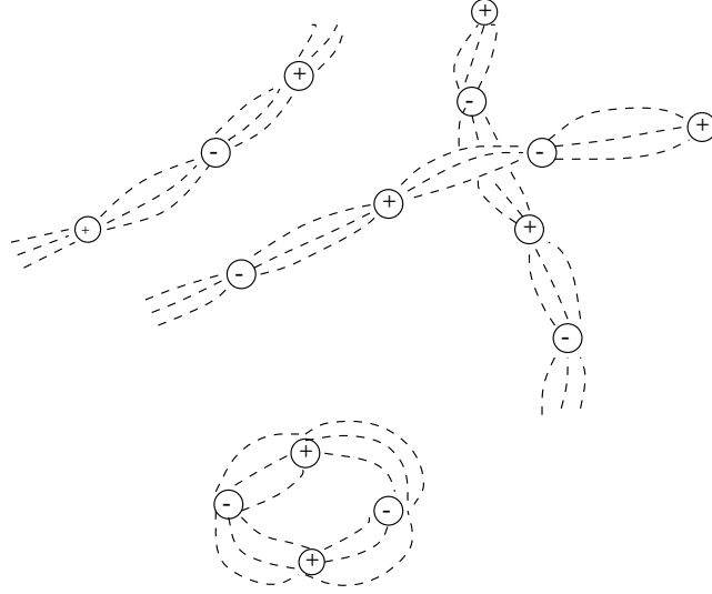
Figure 35: Hypothetical collimation of monopole/antimonopole flux into center vortex tubes on the abelian-projected lattice.
