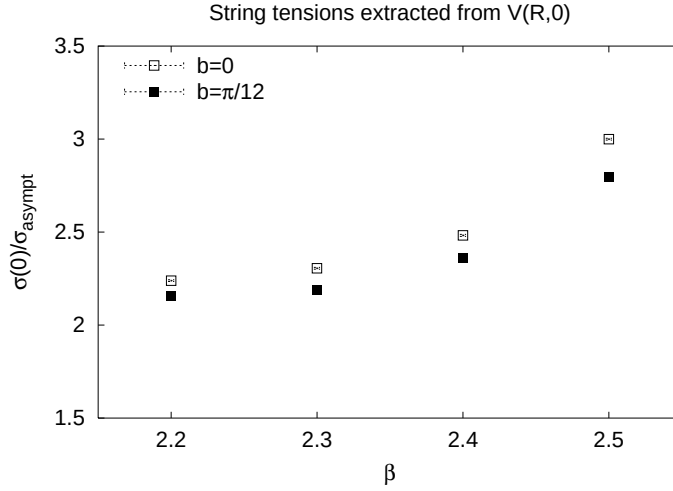
Figure 40: Ratio of \sigma(0)/\sigma , where \sigma(0) \rightarrow \sigma_{Coulomb} in the continuum limit, and \sigma is the usual asymptotic string tension. The string tensions are extracted from fits to a - b/R + \sigma R , with either b = 0 , or the string-motivated value of b = \pi/12 . From Greensite and Olejník, ref. [163].
