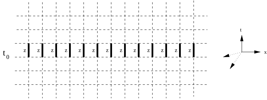
Figure 4: The global center transformation. Each of the indicated links in the t -direction, at t = t_0 , is multiplied by a center element z . The lattice action is left unchanged by this operation.
