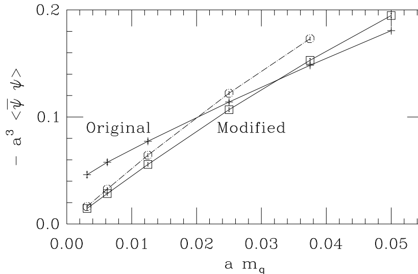
Figure 24: The effect of vortex removal on the chiral condensate in quenched lattice gauge theory. Data points denoted “Modified” are from configurations with vortices removed in DMC gauge (open circles come from a looser gauge-fixing criterion). From de Forcrand and D’Elia, ref. [84].
