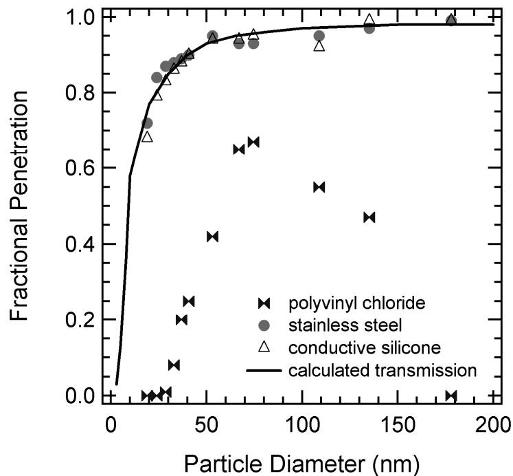
Figure 1. Fractional penetration (transmission) of size selected soot particles through test sections of stainless steel, conductive silicone, and polyvinyl chloride tubing. Fractional penetration is nearly identical for stainless steel, and conductive silicone tubing. Electrostatic losses in the non-conducting polyvinyl chloride tubing greatly reduce particle transmission. The penetration calculated for conductive tubing is shown for reference. Calculated penetration includes losses due to diffusion and inertia (settling), but not electrostatic losses. Conditions: 50 SLPM flow rate, 1.27 cm i.d. tubing, 50m tubing length, 25°C, 1 bar pressure.
