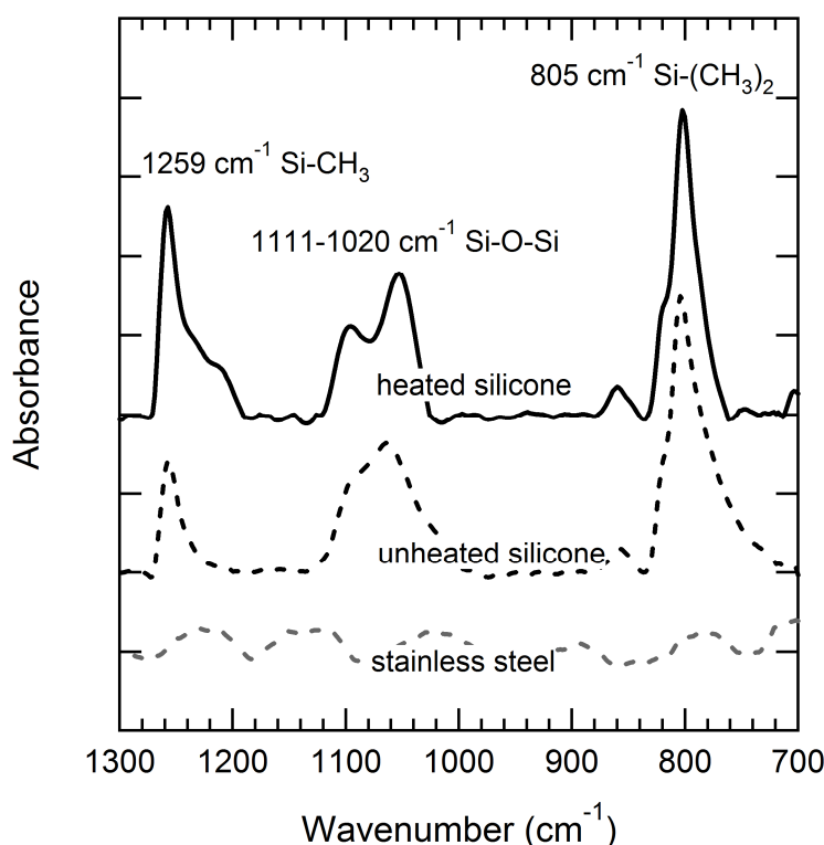
Figure 6. FTIR spectra of soot passed through equal lengths of stainless steel and silicone conductive tubing at room temperature (unheated), and heated silicone conductive tubing. Peaks in the spectra of the soot collected via silicone tubing correspond to siloxane functional groups and are not evident in the spectra of soot collected via stainless steel tubing. The distance between each tick mark on the vertical axis is 0.01 absorbance units.
