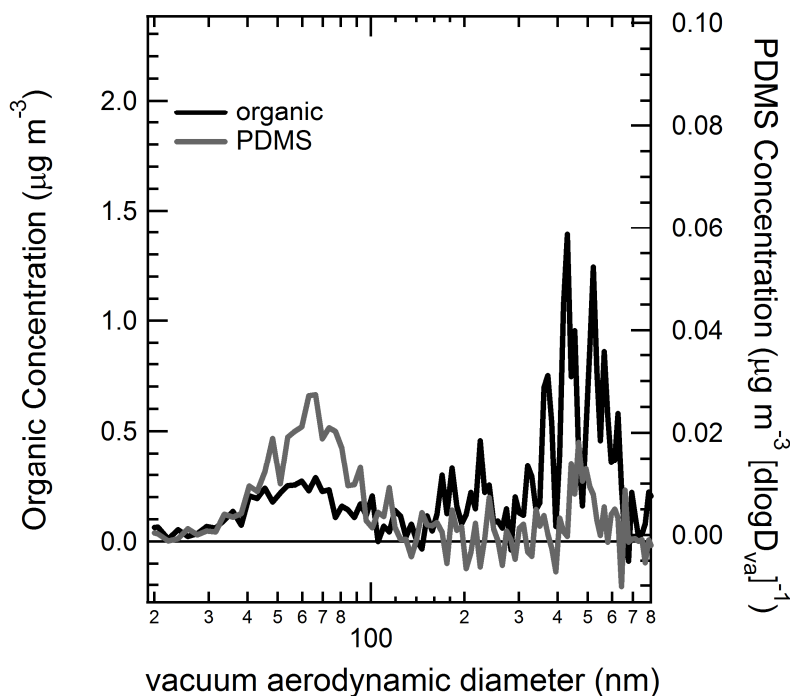
Figure 4. Particle size distribution of organic material and PDMS coated on soot particles generated by combustion of kerosene in a diffusion flame. Data were collected over the course of an hour by an aerosol mass spectrometer. The mass loading of PDMS is about 10% of the total organic material in the 30-100 size range. The size distribution of PDMS and organic material indicates well-mixed particle population for soot sized particles (30-100 nm). Ambient organic aerosol present in the laboratory during the testing period (diameter > 200 nm) has measurable but lower capacity for PDMS compared to the soot particles. The ratio of the organic scale to the PDMS scale is 12:1.
