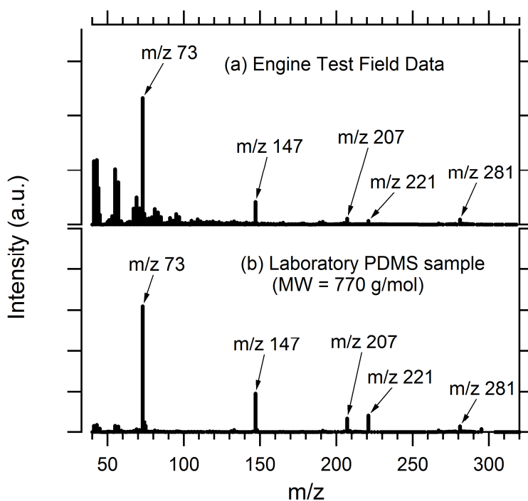
Figure 3. Characteristic EI ionization mass spectra obtained for a) engine exhaust particles and b) aerosolized polydimethylsiloxane (PDMS). The m/z features distinctive of PDMS, ( m/z = 73, 147, 207, 221, 281 ) are readily apparent as a contaminant in the engine exhaust particles.
