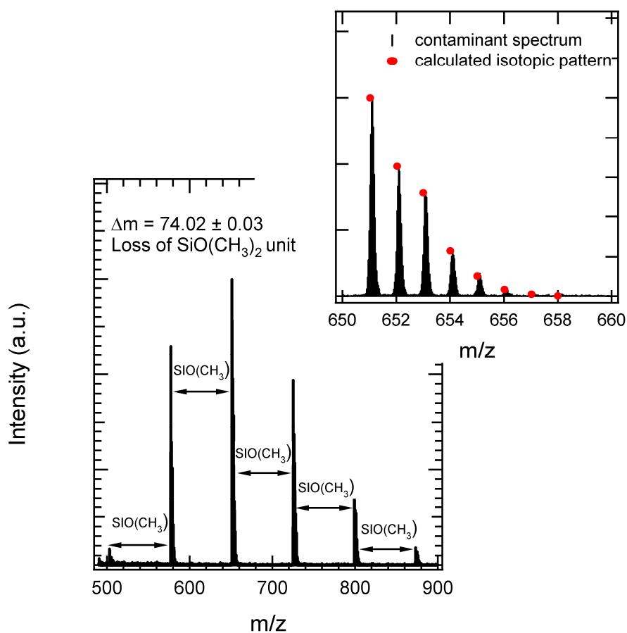
Figure 5. High resolution ( \Delta m/m \sim 3,000 ) mass spectrum for the PDMS contaminant obtained after soft-ionization using VUV radiation. Adjacent peaks are separated by 74.02 \pm 0.03 mass units, which corresponds to SiO(CH_3)_2 ( m/z 74.02). The inset compares the experimental spectrum to the predicted isotopic fragmentation pattern for (SiO(CH_3)_2)_8SiOCH_3^+ .
