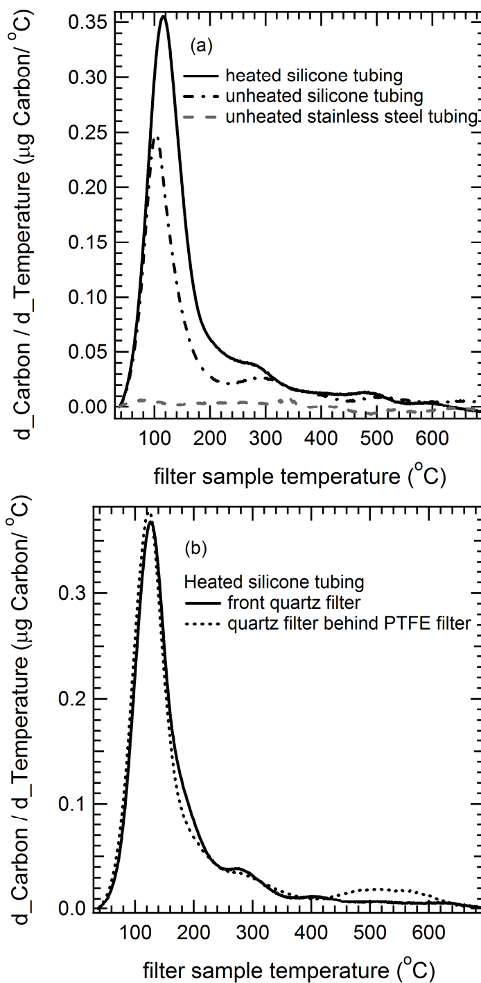
Figure 7. Evolution of carbon as a function of temperature for (a) quartz filters that were used to sample particle free air through heated and unheated silicone conductive tubing and unheated stainless steel tubing and (b) a front and a backup quartz filter collected downstream of heated silicone conductive tubing.
