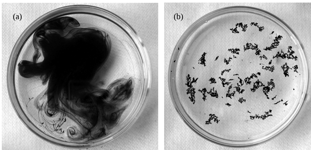
Figure 8. (a) Soot from a diffusion flame made hydrophilic by reaction with ozone. Shown is the soot as it is mixing with water. (b) Soot from a diffusion flame that does not mix with water despite ozone exposure. The soot in (b) was collected through silicone conductive tubing as opposed to the soot in (a), which was collected through stainless steel tubing.
