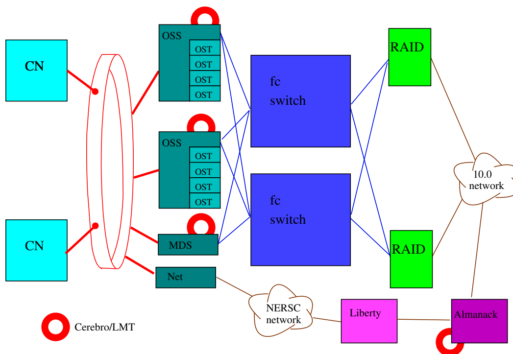
Figure 1: The Franklin Cray XT4 has a SeaStar2 interconnect linking compute nodes (CN) and service nodes (OSS, MDS, Net) in a torus (red links). I/O support is provided by RAID devices connected over 4\text{Gb/s} fibrechannel (blue). External connections to the wider NERSC network are over ethernet (brown). The Cerebro/LMT service resides on the I/O servers (MDS, OSS) and the database server (Almanack).
