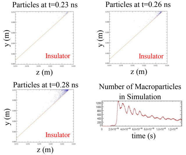
Figure 9. Insulator field emission takes place near the anode triple junction due to field enhancement. As the E-field increases electrons begin to emit further down the insulator towards the cathode.
