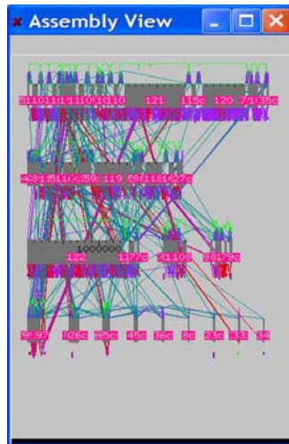
Fig. 3. Draft assembly views of Burkholderia phytofirmans PsJN (GenBank AAUH000000000.)
