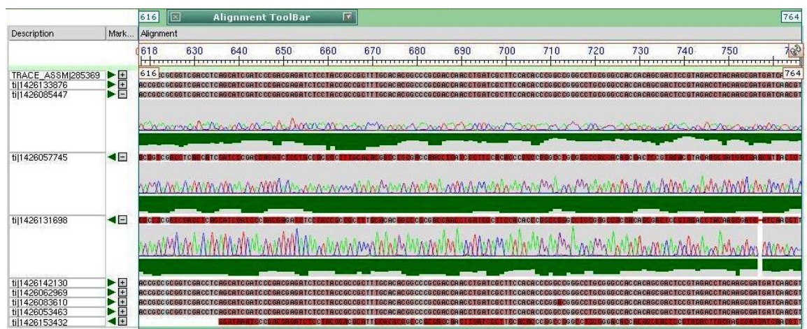
Fig.8. The underlying sequences and Traces from the draft assembly of Salinospora tropica CNB440.
