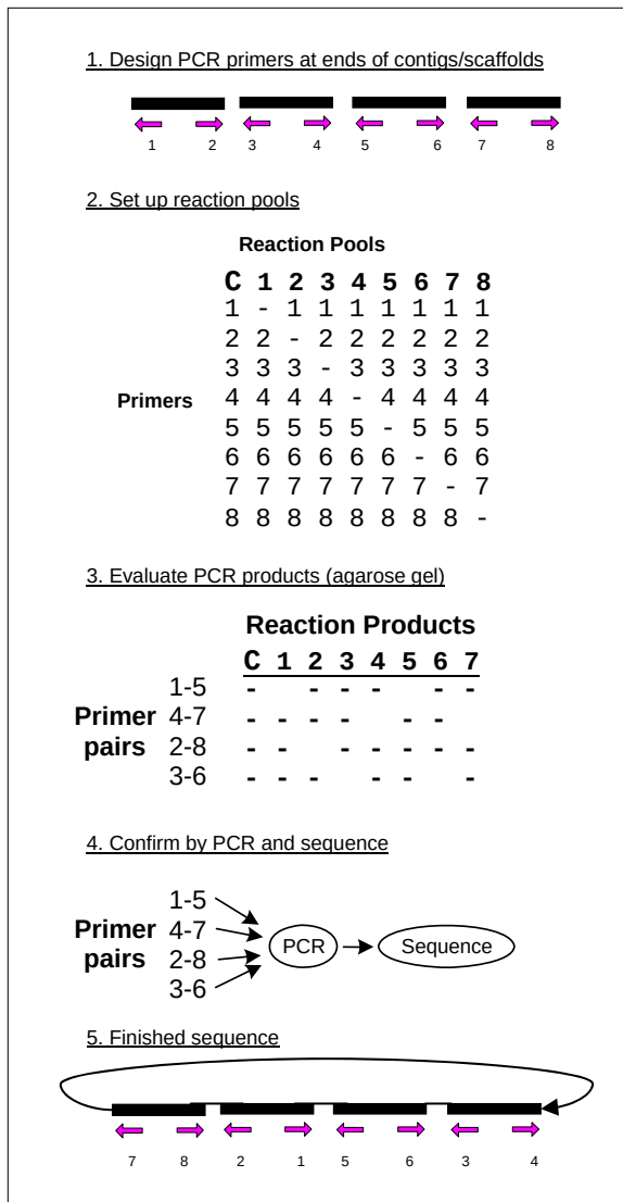
Fig.5. Multiplex PCR approach: schematic representation.
