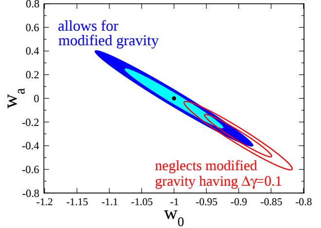
FIG. 1: 68% and 95% CL constraints on the expansion history equation of state parameters w_0 and w_a , marginalized over all other parameters. The two blue (filled) contours give constraints from combining weak lensing, supernovae, cluster, and CMB data, while simultaneously fitting for beyond Einstein gravity. The black dot shows the fiducial model. The two red (empty) contours show the biased constraints if the modified gravity growth rate, here with \Delta\gamma = 0.1 , is ignored (i.e. fixing \gamma to the general relativity value).
