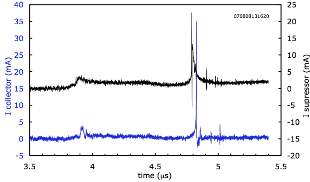
Figure 2: Faraday cup response to uncompressed beam and bunched portion ( t \approx 4.8 \mu\text{s} ).
