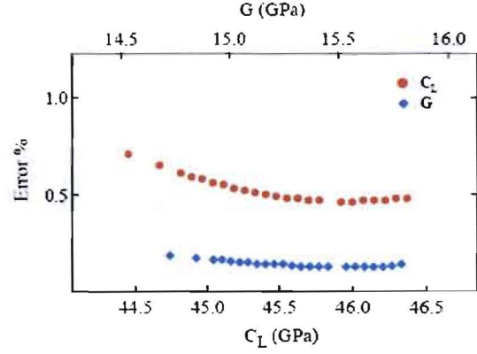
FIG. 4: Chi-square error of shear and longitudinal elastic moduli versus moduli to test for fitting and isotropy errors.
