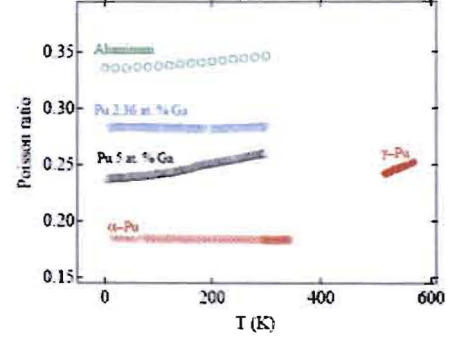
FIG. 7: Comparison of Poisson's ratio versus temperature of aluminum, \alpha -Pu, \gamma -Pu, Pu (2.36 at. % Ga), and Pu (5 at. % Ga).
