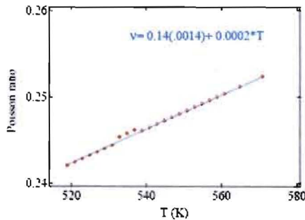
FIG. 6: Temperature variation of Poisson's ratio for \gamma -Pu. The line is a fit of Poisson's ratio versus temperature. The parameters of the fit are given in the figure.
