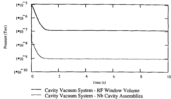
Figure 5: Pump Down Curves from 10^{-5} Torr for the RF Window Volumes and the Nb Cavity Assemblies under Nominal Operating Conditions
