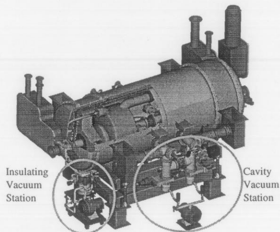
Figure 1: Final Design Layout for the Insulating and Cavity Vacuum Systems
