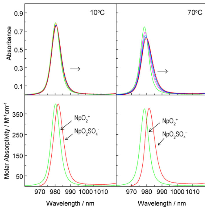
Fig. 1 Representative spectrophotometric titrations of Np(V)/sulfate complexation. I = 1.0 \text{ mol}\cdot\text{dm}^{-3} \text{Na}(\text{ClO}_4/\text{SO}_4) . Upper figures – normalized absorption spectra collected in the titration at 10 and 70°C. Titrant: 0.500 \text{ mol}\cdot\text{dm}^{-3} \text{Na}_2\text{SO}_4 . C_{\text{Na}_2\text{SO}_4} = 0 - 0.1875 \text{ mol}\cdot\text{dm}^{-3} in the titration. Initial solution in cuvette: 2.50 mL; 5.124 \times 10^{-3} \text{ mol}\cdot\text{dm}^{-3} \text{NpO}_2\text{ClO}_4/1 \times 10^{-6} \text{ mol}\cdot\text{dm}^{-3} \text{HClO}_4 (10°C), 5.00 \times 10^{-3} \text{ mol}\cdot\text{dm}^{-3} \text{NpO}_2\text{ClO}_4/1 \times 10^{-6} \text{ mol}\cdot\text{dm}^{-3} \text{HClO}_4 (70°C). Lower figures – calculated molar absorptivity of \text{NpO}_2^+ , and \text{NpO}_2\text{SO}_4^- at 10 and 70°C.
