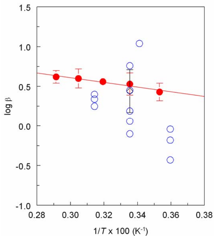
Fig. 2 \log \beta vs. 1/T for the complexation of U(VI) with sulfate. Solid symbols (●): experimental data from this work ( I = 1.0 \text{ mol}\cdot\text{dm}^{-3} \text{ Na(ClO}_4\text{/SO}_4\text{)} ); Open symbols (○): experimental data in the literature ( I varies from 0.5 - 2.2 \text{ mol}\cdot\text{kg}^{-1} \text{ Na(ClO}_4\text{)} [2]; (◇): NEA selected value of \log \beta^0 [2].
