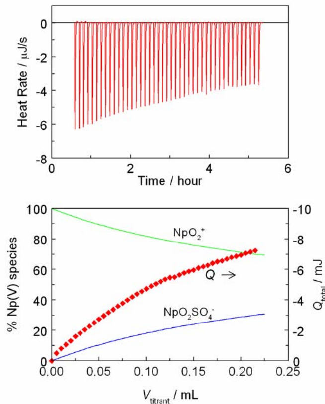
Fig. 3 Calorimetric titration of Np(V) sulfate complexation. I = 1.0 \text{ mol}\cdot\text{dm}^{-3} \text{ Na}(\text{ClO}_4/\text{SO}_4) , t = 40^\circ\text{C} . Cup: 0.900 \text{ mL } C_{\text{Np}} = 1.72 \times 10^{-3} \text{ mol}\cdot\text{dm}^{-3} , C_{\text{H}} = 3 \times 10^{-7} \text{ mol}\cdot\text{dm}^{-3} ; titrant: 0.500 \text{ mol}\cdot\text{dm}^{-3} \text{ Na}_2\text{SO}_4 , 5 \text{ }\mu\text{L}/\text{addition} .
