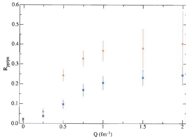
FIG. 3: (Color online) The ratio of pp to pn pairs integrated over relative momentum \mathbf{q} \parallel \mathbf{Q} of 1.5 to 2.5 \text{fm}^{-1} as a function of total momentum Q ; red triangles are for {}^3\text{He} and blue squares for {}^4\text{He} .
