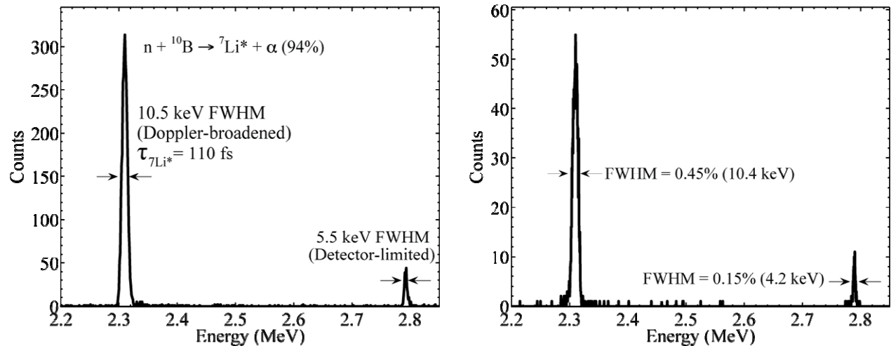
Fig. 5. Thermal neutron spectra of a TES with a \text{TiB}_2 absorber using an optimum filtering routine (left) and using the Pixie-16 algorithm (right). The 2.31 MeV line is Doppler-broadened by the decay of the ^7\text{Li}^* nucleus during thermalization.
