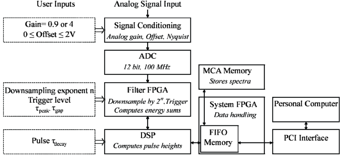
Fig. 1. Block diagram of the Pixie-16 system.
