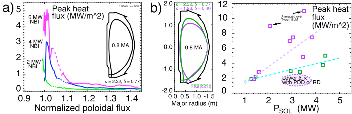
Figure 1: (a) Divertor heat flux profiles measured in similar 0.8 MA plasmas with 2, 4, and 6 MW NBI, (b) Divertor peak heat fluxes measured at different SOL power levels in low and highly shaped plasmas.
