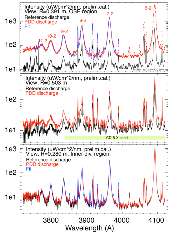
Figure 6: Divertor UV spectra in reference and PDD discharges.
