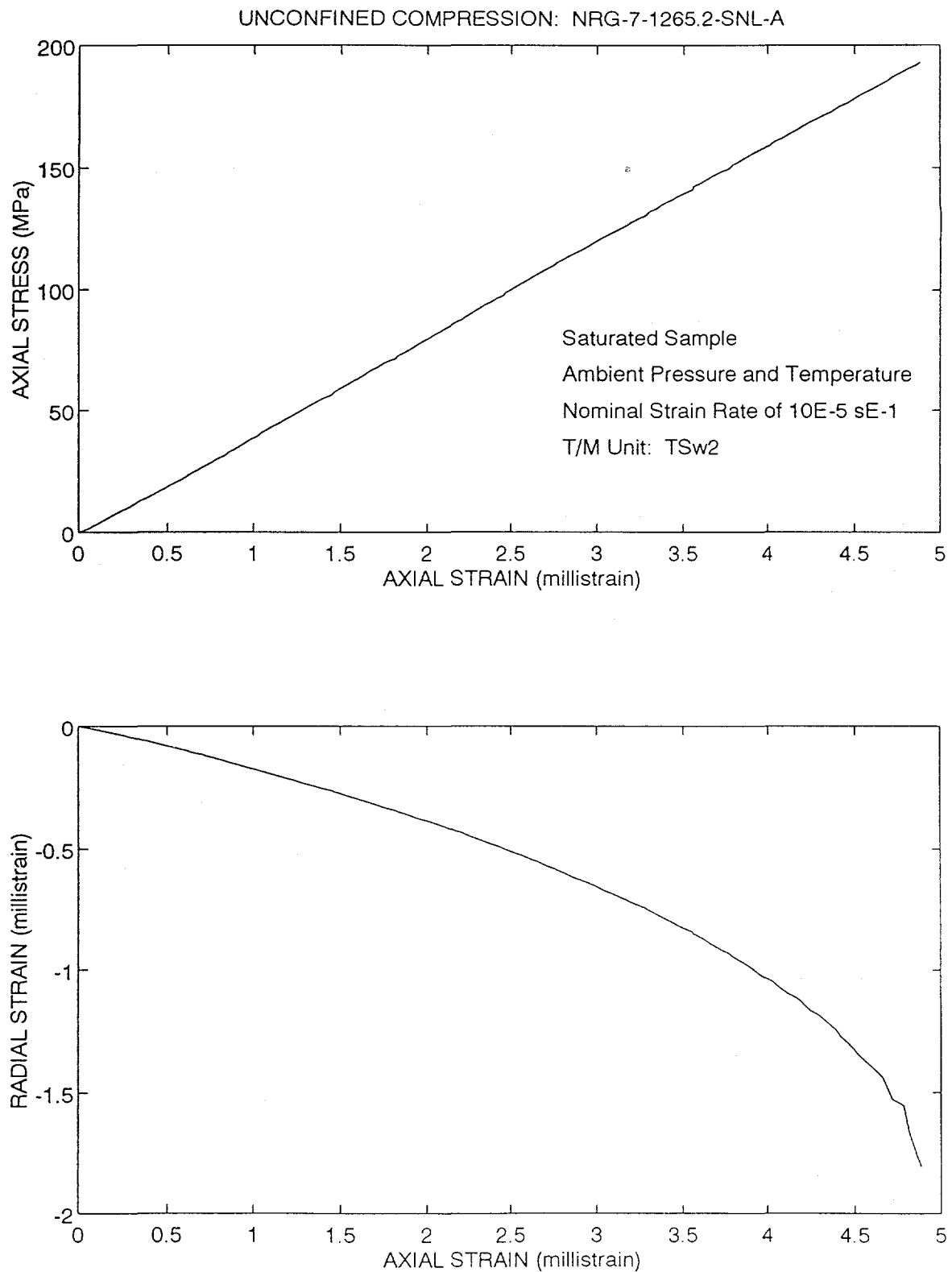
Figure 15. Axial stress and radial strain are plotted as a function of axial strain for an unconfined compression experiment performed on a specimen of TSw2. The specimen was recovered from a depth of 1265.2 feet from borehole USW NRG-7/7A, Yucca Mountain, NV.
