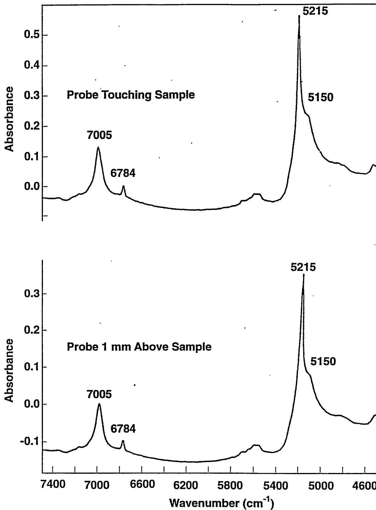
Figure 7. NIR Spectra of Freeze-Dried Sludge.
