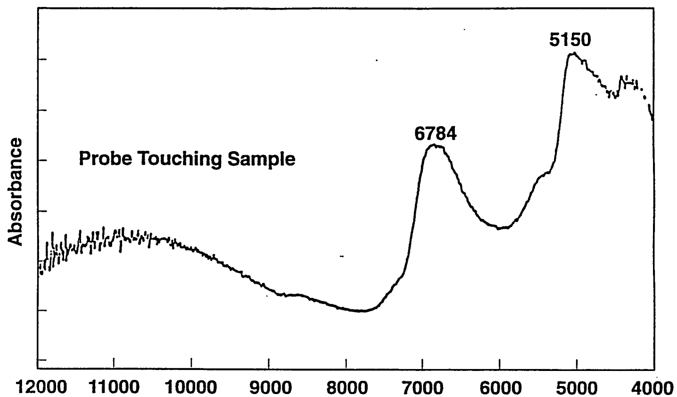
Figure 6. NIR Spectra of Wet Sludge.
