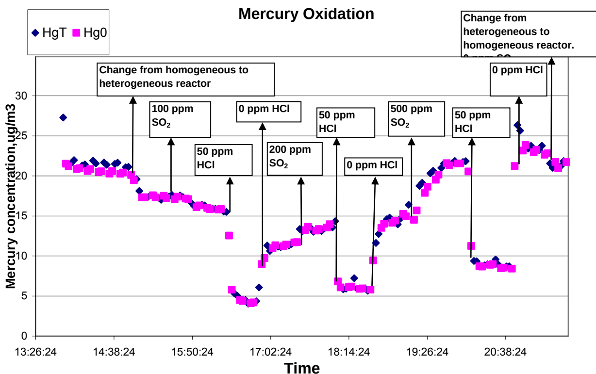
Figure 3 Elemental ( \text{Hg}^0 ) and total ( \text{Hg}^{\text{T}} ) mercury concentrations at the exit of the carbon bed as a function of time (hours) at a temperature of 150^\circ\text{C} at \text{SO}_2 concentrations of 100, 200, 500 ppm and a chlorine concentration of 50 ppm (as \text{HCl} equivalent).
