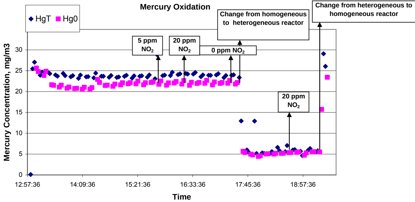
Figure 6 Elemental (Hg 0 ) and total (Hg T ) mercury concentrations at the exit of the carbon bed as a function of time (hours) at a temperature of 150°C at NO 2 concentrations of 5 and 20 ppm.
