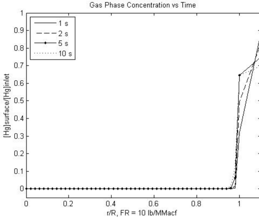
Figure 17 Mercury uptake normalized with inlet concentration over time using Freundlich isotherm model.
