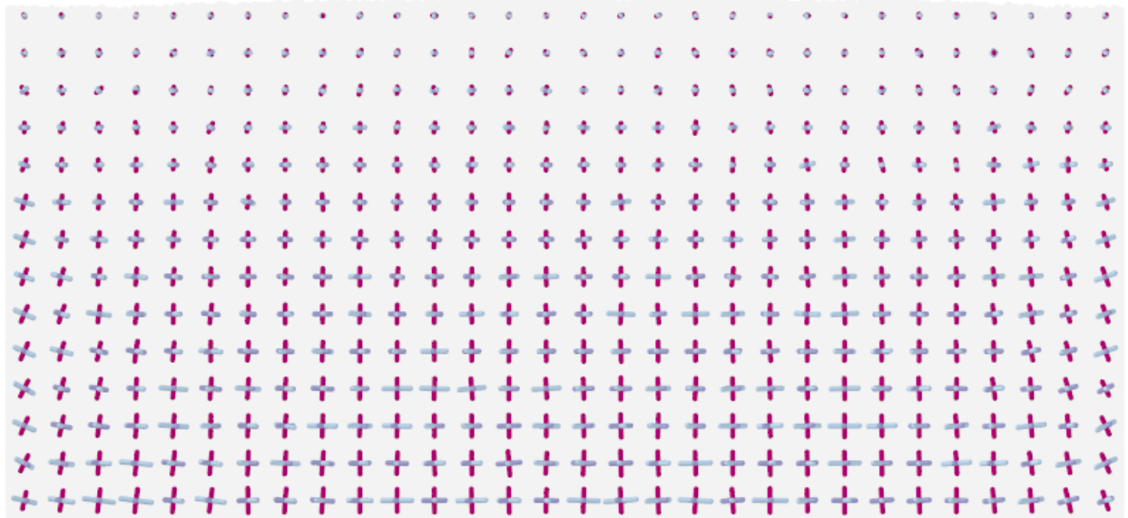
Figure S1: Plots of the directions and magnitudes of the eigenvectors of the deviatoric stress tensors for the wide initial packing.
