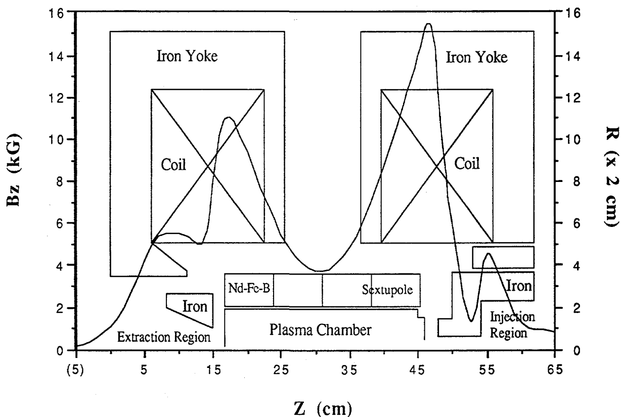
Fig. 4 The conceptual design of the upgraded AECR source. At dc power of 75 kW and with iron plugs to concentrate the field flux, the maximum peak field strengths on axis will reach 1.5 and 1.1 Tesla at the injection and extraction region respectively. In addition, a set of new NdFeB permanent sextupole magnet will increase the maximum radial field strength at the wall to 1 Tesla.
