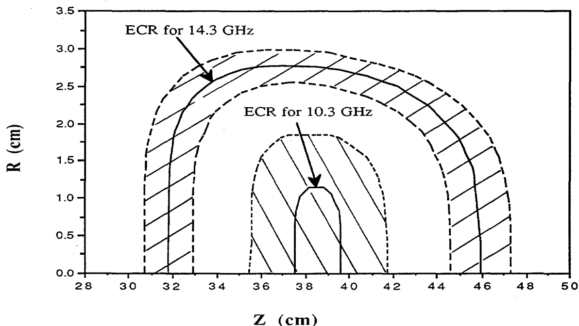
Fig. 2 Approximated heating zones (hatched regions), by assuming the electrons have 2 keV energy along the field lines, for 10.3 and 14.3 GHz in the AECR source with the magnetic field configuration for the best performance on uranium. It indicates that there are two well separate heating zones in the AECR plasma.
