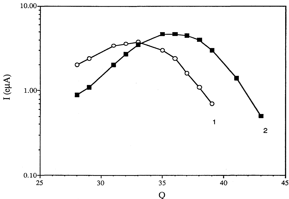
Fig. 1 Charge state distributions for ^{238}\text{U} produced with the AECS source are shown for two cases. Curve 1 indicates the best distribution obtained with single-frequency (14 GHz, at power of 1540 W) heating. Curve 2 shows the distribution obtained with two-frequency (14 + 10 GHz, at a total power of 1770 W with 1480 W of 14 GHz and 290 W of 10 GHz) heating. The peak charge state shifts from 33+ in curve 1 to 36+ in curve 2.
