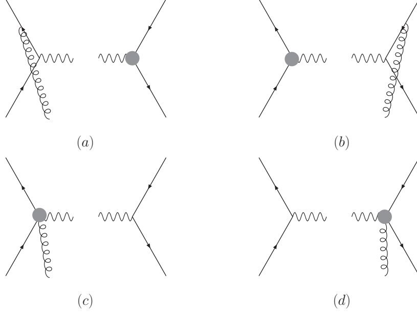
FIG. 2: One-loop virtual correction to the weighted cross section: the gluon attaches to the opposite side of the loop correction (upper two diagrams); the gluon attaches to the same side of the loop corrections (lower two diagrams).
