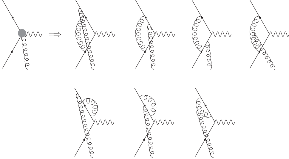
FIG. 4: Corrections to the quark-antiquark-photon vertex with gluon attachment, corresponding to the blob in the lower two diagrams of Fig. 2.
