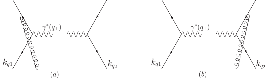
FIG. 1: Leading order contribution to the weighted transverse spin-dependent cross section.
