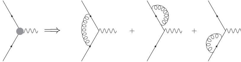
FIG. 3: Corrections to the quark-antiquark-photon vertex, corresponding to the blob in the upper two diagrams of Fig. 2.
