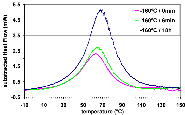
Fig. 2. DSC scans of the \alpha' \rightarrow \delta reversion at -160°C with no holding time and with holding times of 6 minutes and 18 hours. The amount of \alpha' formed during the 20°C/min quench and any additional \alpha' formed during heating are lower than the amount of \alpha' formed during the 18 hour isothermal hold.
