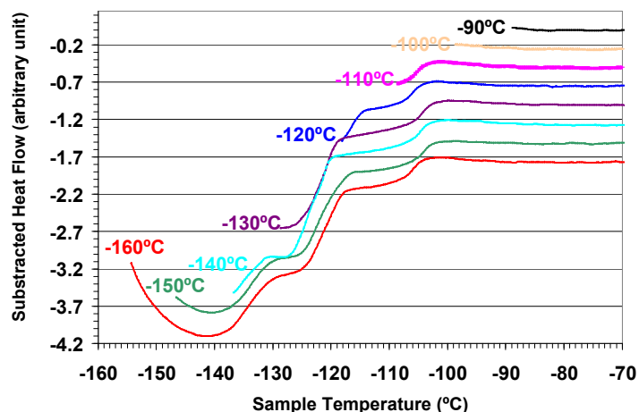
Fig. 3. DSC thermograms corresponding to the \delta \rightarrow \alpha' transformation during continuous cooling at 20°C/min before each 18-hour anneal. This transformation is exothermic and begins at approximately -100°C. The DSC data indicates that the transformation results in 3 overlapping exothermic peaks. The data have been offset along the y-axis for clarity.
