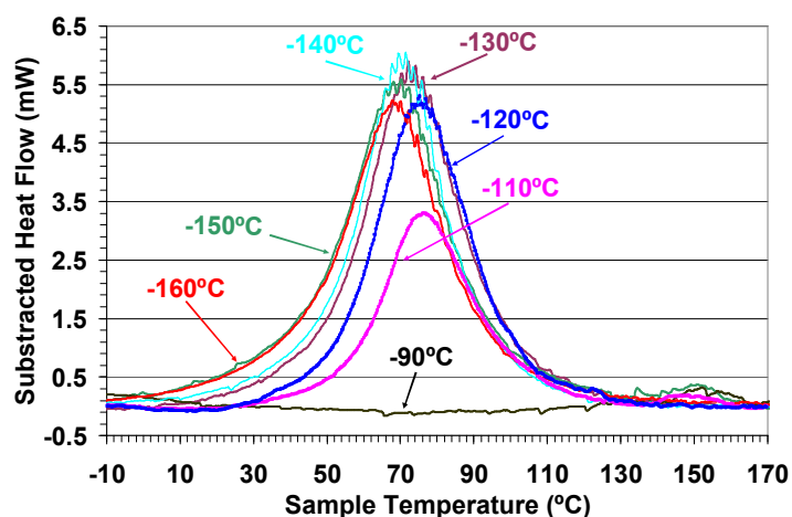
Fig. 4. DSC thermograms corresponding to the \alpha' \rightarrow \delta reversion upon continuous heating at 20°C/min following each 18-hour isothermal hold. The temperatures on the plot correspond to the isothermal holding temperatures. This transformation is endothermic and begins at approximately 25°C.
