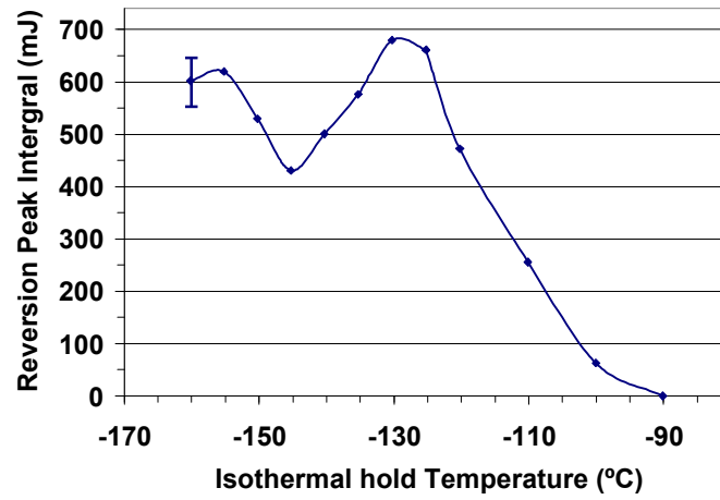
Fig. 5. Integrated peak areas of the \alpha' \rightarrow \delta reversion peaks following 18-hour isothermal holds versus holding temperature. The amount of \alpha' formed is directly related to the integrated area of the \alpha' \rightarrow \delta reversion peak.
