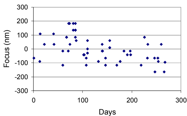
Fig. 8. Focus tracking data obtained from a periodically performed baseline process on the SEMATECH Berkeley MET tool. Day-to-day rms stability is 90 nm.
