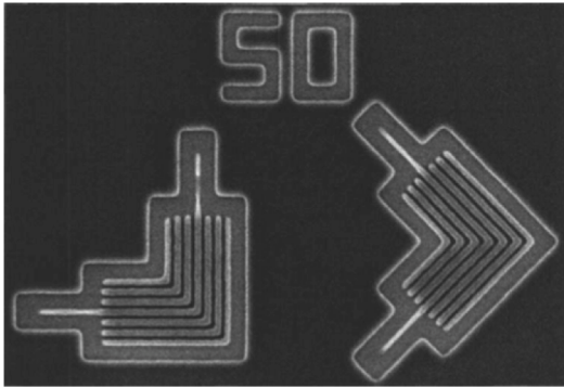
Fig. 5. Scanning electron microscope (SEM) image of the printed elbow features used to extract the astigmatism data. The 0^\circ and 45^\circ -oriented elbow patterns are placed in close proximity on the mask to ensure that dose and focus can be assumed constant over the features of interest.
