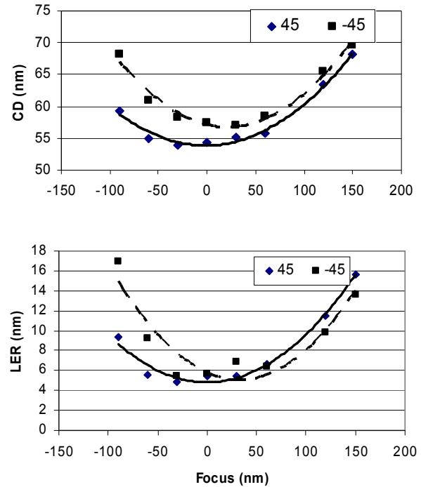
Fig. 6. Through-focus CD and LER data with quadratic fits for one field point representative of the 3 \times 1 grid of measured central field points. The -45^\circ and 45^\circ feature data is shown, corresponding to 45^\circ astigmatism.
