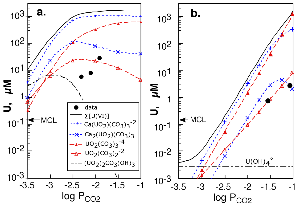
Figure 4. Calculated effects of increased \text{CO}_2 partial pressure from OC oxidation under (a.) oxidizing conditions ( \text{pe} = 11.96 , \text{Ca}^{2+} = 2.0 mM), and (b.) reducing conditions ( \text{pe} = -3.23 to -3.35 , \text{Ca}^{2+} = 0.4 mM, equilibrium with \text{UO}_2(\text{am}) ). Only concentrations of dominant species and total calculated U are plotted for comparison with trends in measured U concentrations. Under both conditions, increased P(\text{CO}_2) allows higher aqueous U concentrations.
