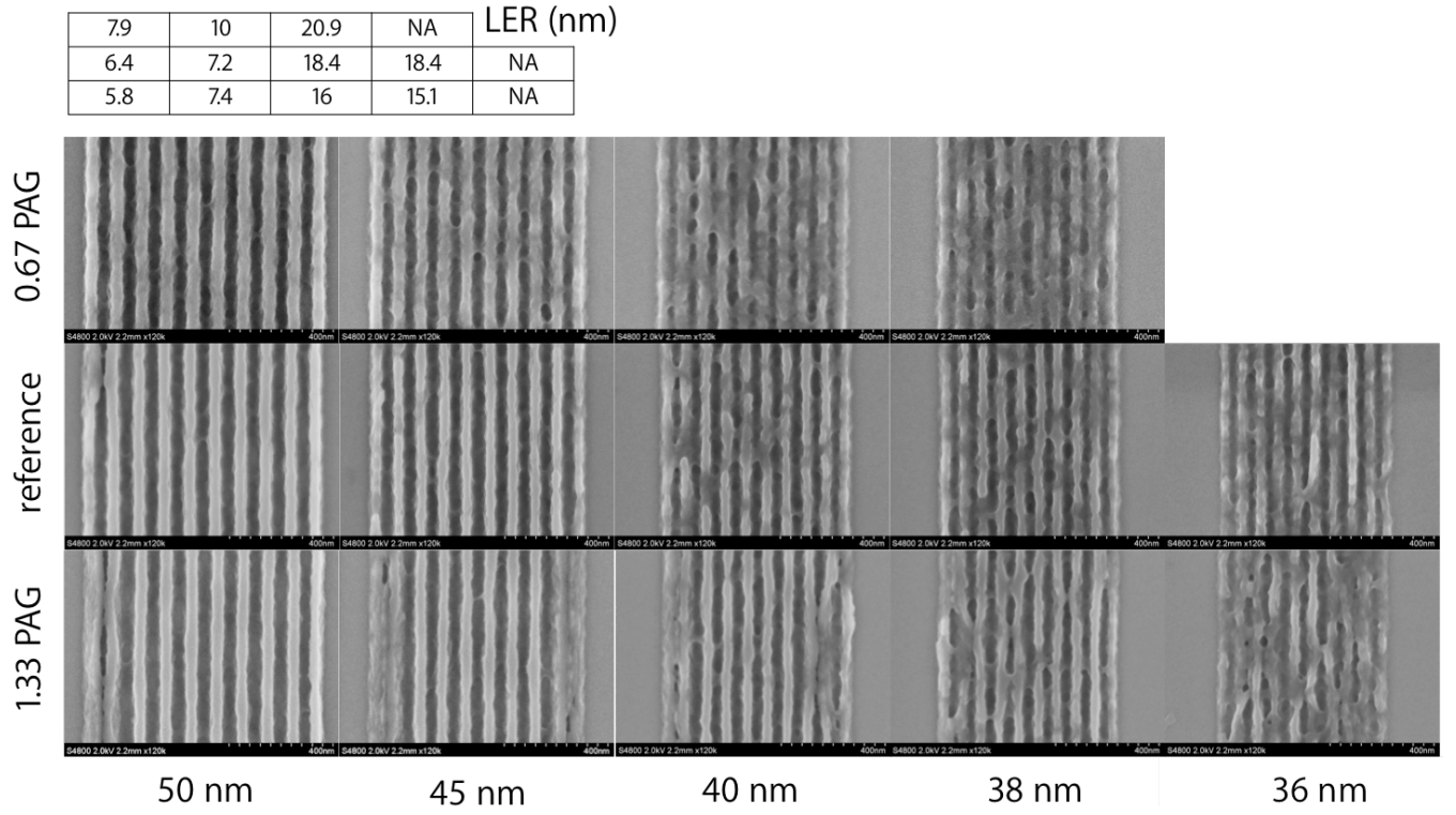
FIG. 2: Photo-acid generator (PAG) study. Through-pitch SEM images of bright field 1:1 lines printed in EH27 resist. Relative PAG weight percents are indicated to the left of each row. Half-pitch coded feature sizes are indicated at the bottom of each column. LER information for each SEM image is indicated in the table.
