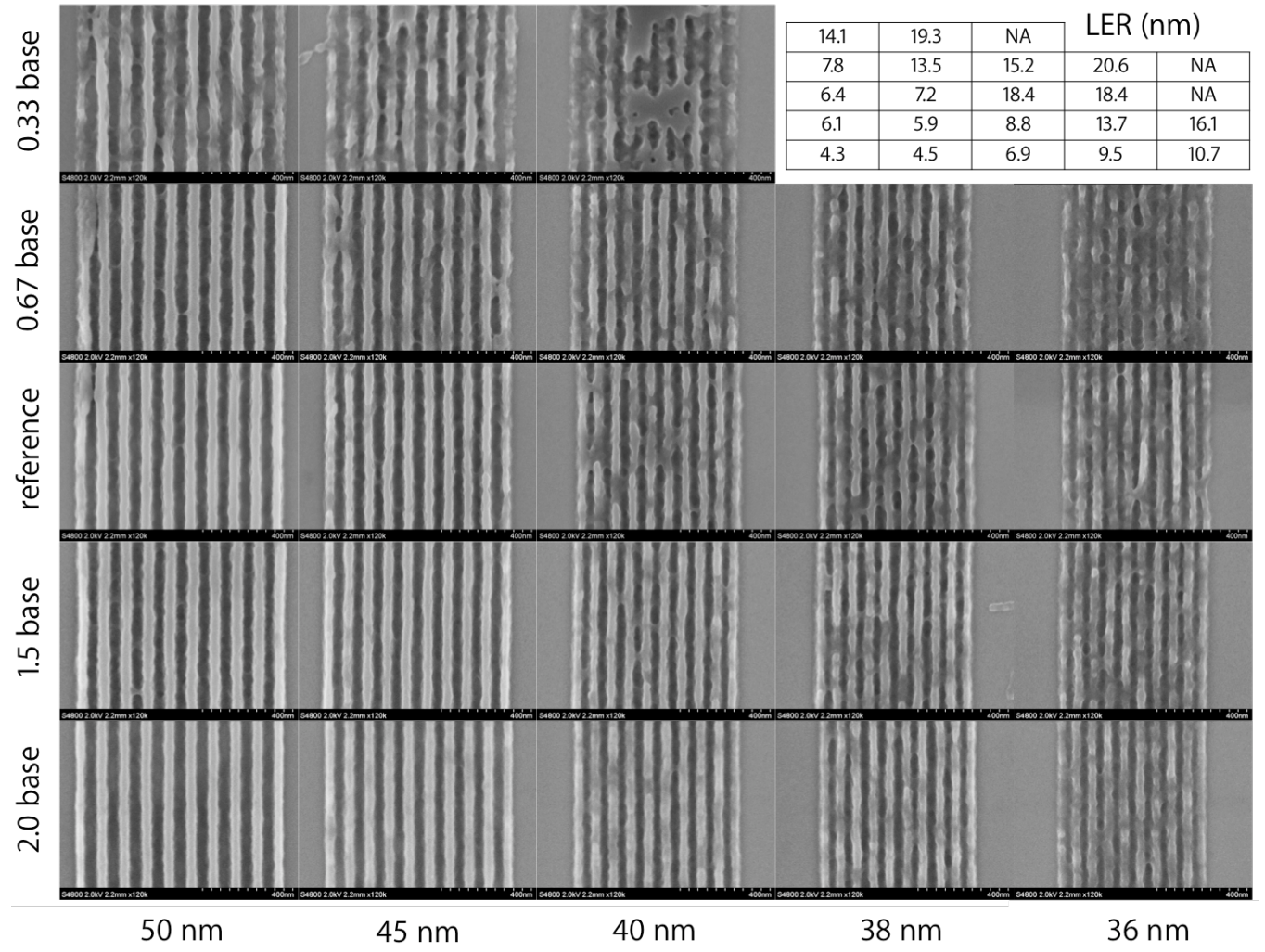
FIG. 1: Base loading study. Through-pitch SEM images of bright field 1:1 lines printed in EH27 resist. Relative base weight percents are indicated to the left of each row. Half-pitch coded feature sizes are indicated at the bottom of each column. LER information for each SEM image is indicated in the table.
