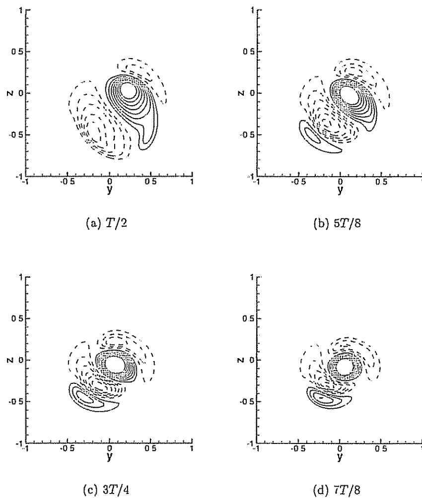
Figure F.7: Spinning sphere at Re = 300 , oblique rotation: shedding cycle, stream-wise vorticity in the x = 2 plane (continued)
