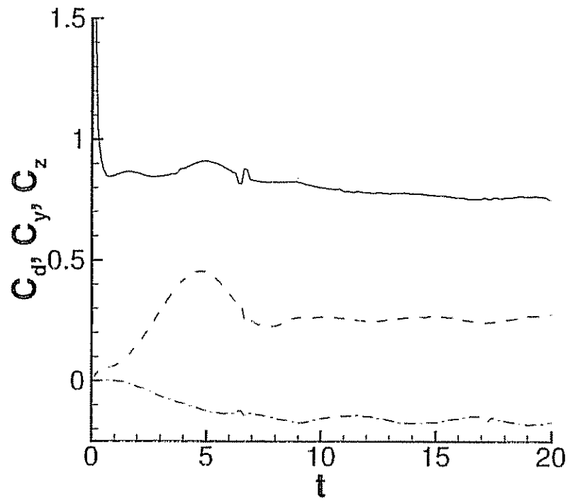
Figure 6 32: Spinning sphere at Re = 300 , oblique rotation: drag coefficient C_d (solid), lift coefficient C_z (dashed) and transverse force coefficient C_y (dash-dotted)
