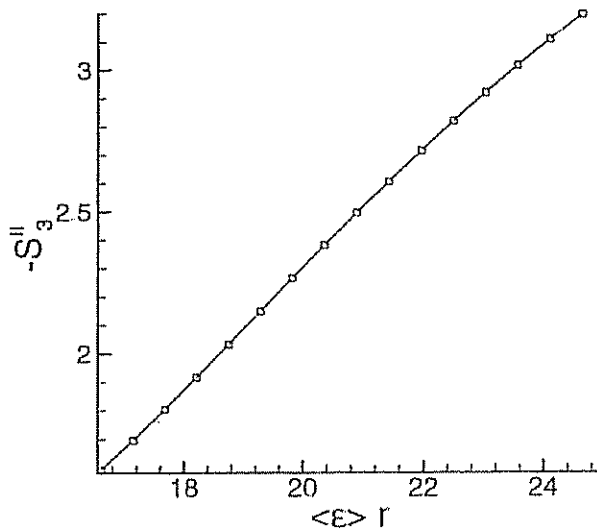
FIG. 4. Third order velocity structure function at stoppage time t_e = 0.14 ; the actual r interval is [0.4, 0.6] .
