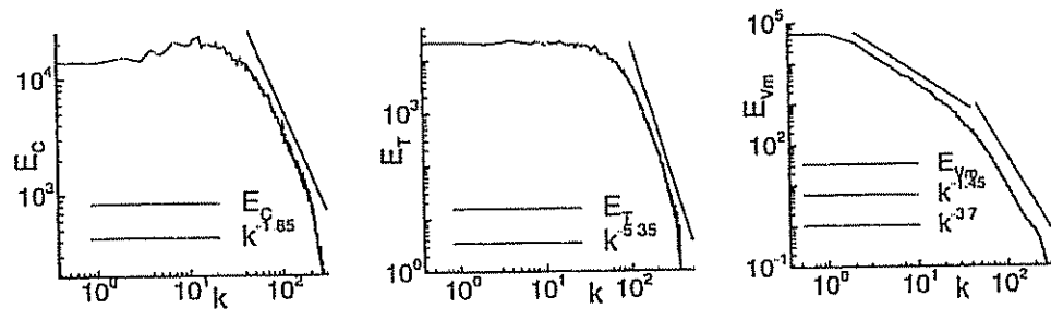
Fig. 4. Spectra of curvature E_C , torsion E_T and Lagrangian velocity E_{v_m} .
