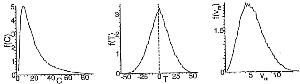
Fig. 3. Histograms of curvature C , torsion T and length of Lagrangian velocity v_m = \|V_m\| at stoppage time. The frequencies are shown divided by 10^3 . The number of sample points is approximately 7 \times 10^4 .
