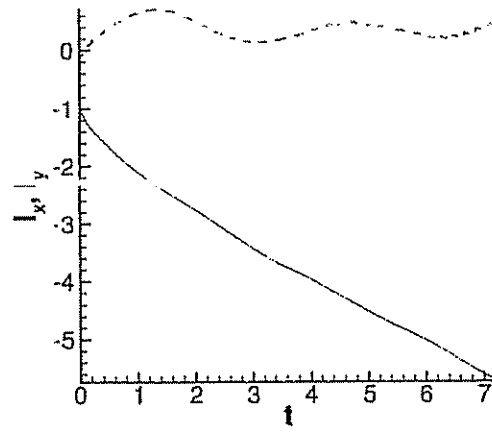
Figure 7.3: Swimming fish at Re_{U_\infty} = 100 , f = 0.25 : flow momentum; stream-wise momentum I_x is solid, transverse I_y is dashed
