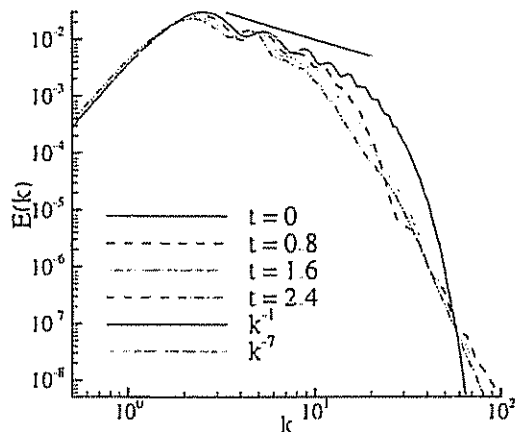
FIG 4. Vortex rings in an offset collision: evolution of the energy spectrum
