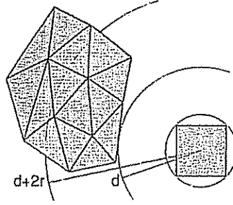
FIG 6.1 Illustration of Least Upper Bound criterion. Only faces whose shortest distance from the cell center is less than or equal to d_{\min} + 2r need be considered; the outer three triangles can be safely ignored
