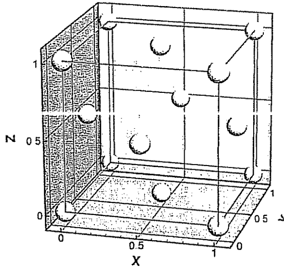
Figure 2 2: Face-centered cubic lattice: unit cell
