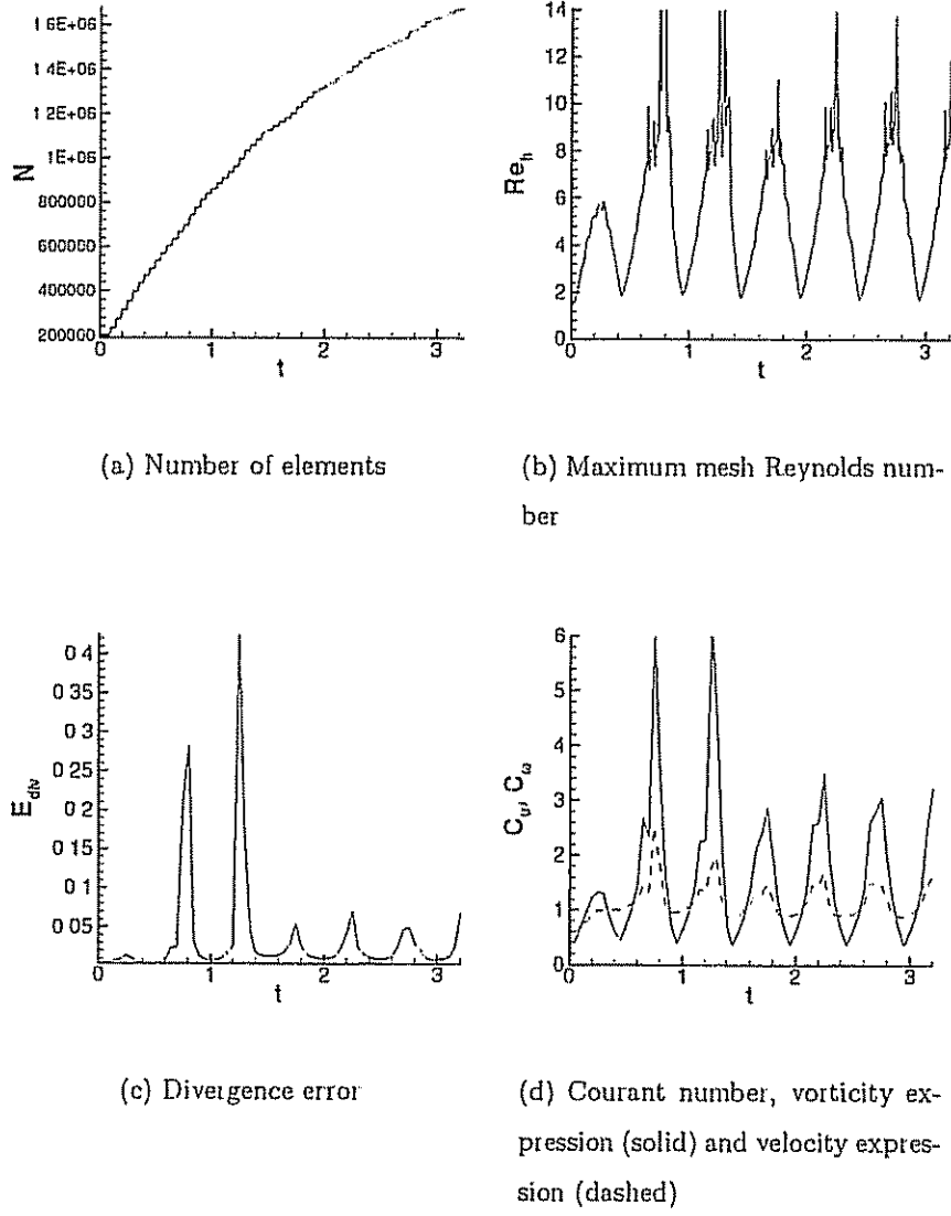
Figure 7.6: Swimming fish at Re_{U_\infty} = 100 , f = 1 : numerical diagnostics
