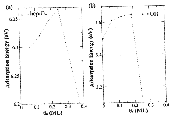
FIG. 3. Adsorption energy of (a) O_{ads} and (b) OH as a function of \theta_0 on O/Ru(0001) surfaces.
