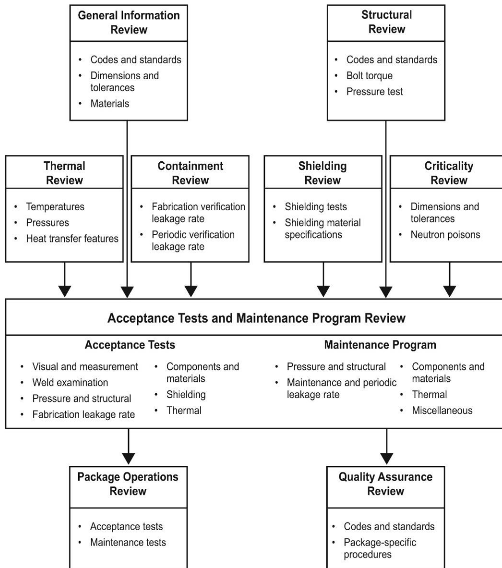
Figure 8.1 Example of Information Flow for the Acceptance Tests and Maintenance Program Review
