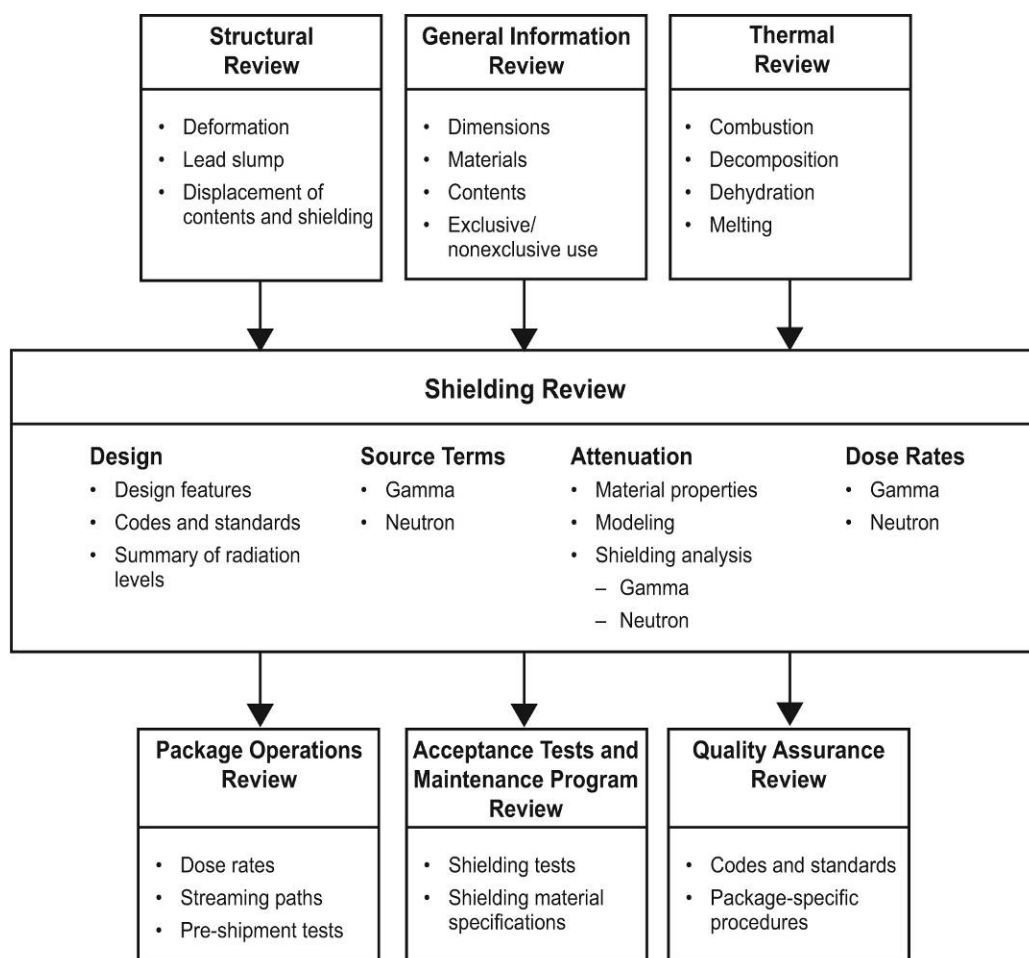
Figure 5.1 Example of Information Flow for the Shielding Review
