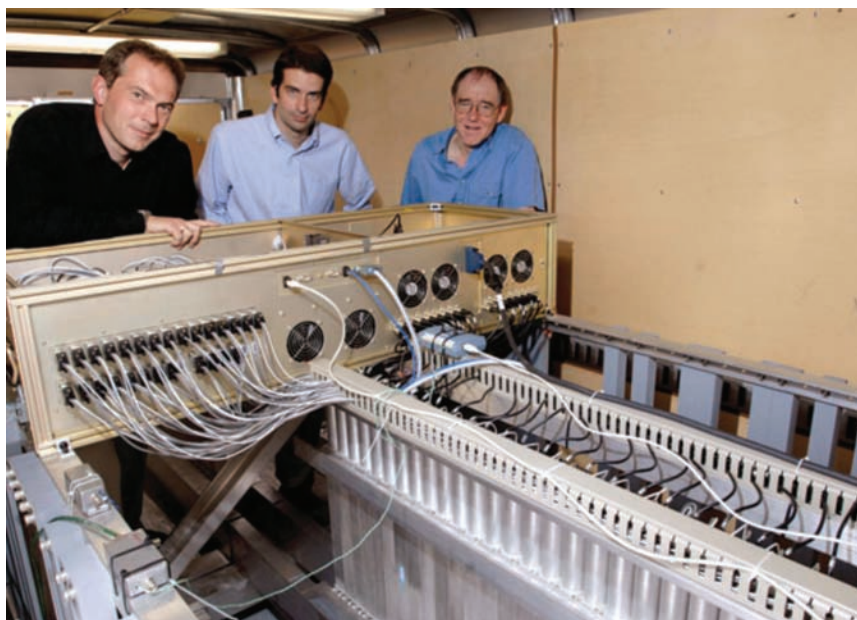
Lorenzo Fabris, Thomas Karnowski, and Klaus Ziock (left to right) and the large-area imager.
