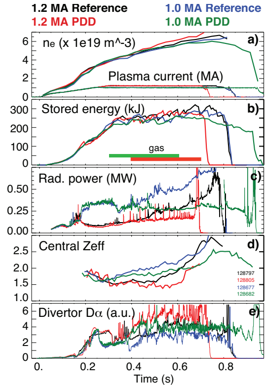
Figure 2: Time traces of 1.0 MA and 1.2 MA 6 MW discharges with and without divertor gas injection.
