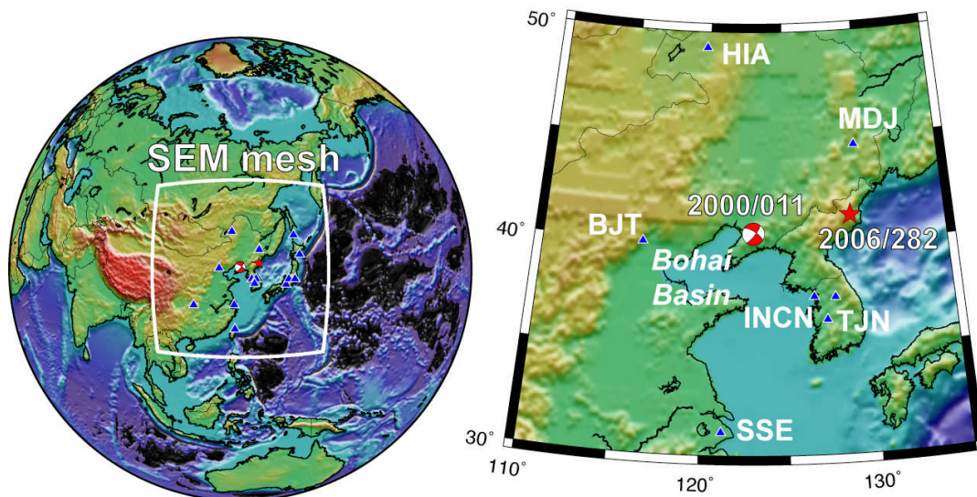
Figure 1. (left) SPECFEM3D computational domain for regional simulations of events in East Asia. (right) Map showing the locations of the January 11, 2000 (2000/011) earthquake and October 9, 2006 (2006/282) North Korean nuclear explosion along with regional broadband stations that recorded the events.
