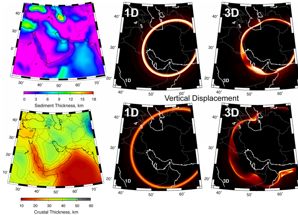
Figure 4. WENA 3D model properties across the Middle East: sediment thickness (top left) and crustal thickness (bottom left). Snapshots of vertical ground displacements showing Rayleigh wave propagation for an isotropic source using an average 1D model (center) and the WENA 3D model (right).
