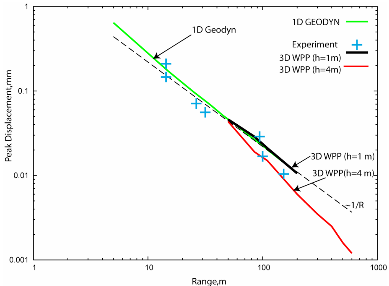
Figure 9. Peak displacement versus range for a chemical high-explosive (HE) source in a limestone whole-space: experimentally measured values (crosses) from Figure 8 of Murphy et al. (1997); calculated with 1D GEODYN (solid green line); and calculated with 3D WPP (red line for 4 m grid spacing and black line for 1 m grid spacing). These are compared with the expected geometric spreading for a spherical wave in a homogeneous whole-space ( 1/R , fine dashed line).
