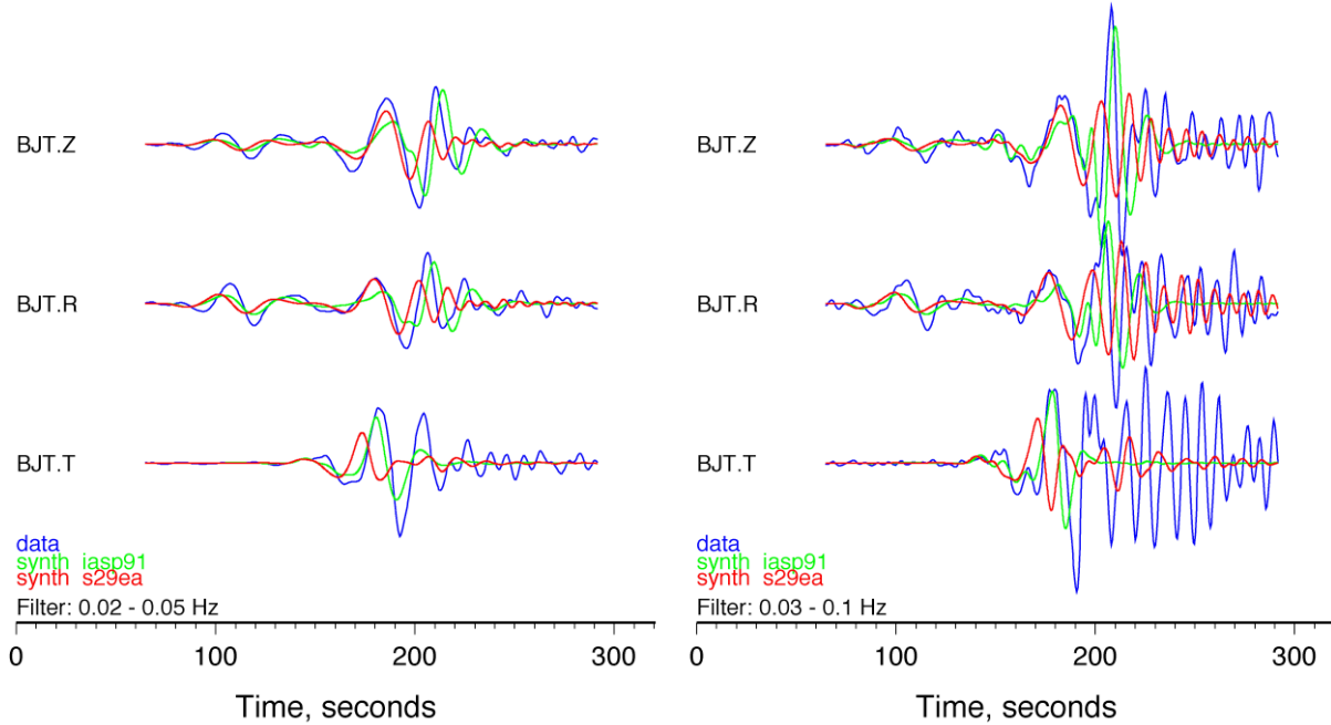
Figure 2. Observed (blue) and synthetic seismograms for the 2000/011 earthquake at station BJT for the iasp91 (green) and s29ea + CRUST2.0 (red) models filtered 0.02-0.05 Hz ( left ) and 0.03-0.1 Hz ( right ).
