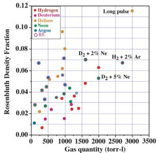
Fig. 9. Rosenbluth density fractions for MEDUSA MGI. Violet “RE” umbra denotes examples with runaway electron production.
