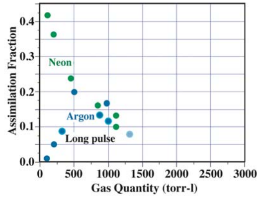
FIG. 11. High-Z data from Fig. 9, interpreted as an assimilation fraction.
