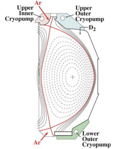
FIG. 1. Particle pumping and gas injection locations are shown together with the cross-section of a DN plasma.
