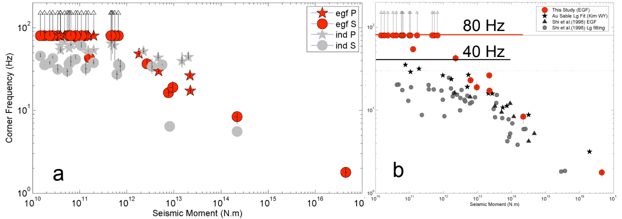
Figure 4. Corner frequency measurements and comparison with previous work in eastern North America. (a) compares the EGF and individual fitting results for P and S wave measurements, averaged for each earthquake. The agreement is good for larger magnitudes, but the individual method underestimates the corner frequency when it nears the maximum frequency limit. (b) Comparison of our results with those of Shi et al. (1998). The concluded that scaling broke down below M_0 \sim 10^{13} Nm, but comparison with our results implies that this is an artifact of their lower maximum frequency limit (40 Hz), and use of only individual fitting results for the smaller earthquakes.
