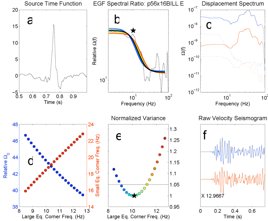
Figure 3: Example of analysis to obtain parameters from spectral ratio. (a) shows the source time function, (b) the spectral ratio of the displacement spectra (black) and the fits (rainbow colors) within 5% increase of variance of the minimum. The star marks the corner frequency of the minimum variance fit. (c) the displacement spectra of the two earthquakes (solid) and their preceding noise (dotted). (d) the long period amplitude of the ratio, and corner frequency of small earthquake, as the corner frequency of the large earthquake is varied, (e) the variance of the fit, colors are the same as in (b), and (f) the raw P wave seismograms with the relative amplification of the smaller (red) earthquake used in the plot. In this example a M \sim 3 is divided by a M \sim 2 , and the seismograms are highly correlated, we have a clear source time function, a tight parabola in variance, and two well resolved corner frequencies
