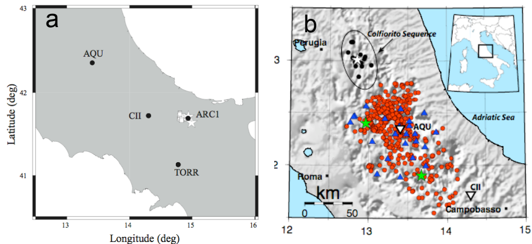
Figure 1: Maps of (a) the San Giuliano and (b) the Colfiorito earthquake sequences. In (a) main shocks are indicated by white stars, aftershocks by white squares, and seismic stations by black solid circles. In (b) the earthquakes used are shown as black dots, and the stations as inverse white triangles.
