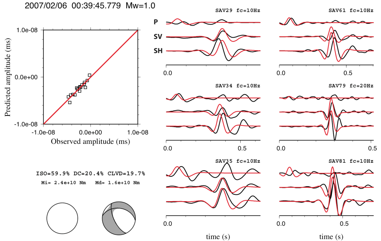
Figure 6. Moment tensor inversion results for a M_w=1.0 event recorded at Savuka mine. (left) Comparison between observed and predicted spectral amplitudes and isotropic and deviatoric “beach-balls” for the moment tensor. (right) Comparison of observed (black) and predicted (red) waveforms. Realize the inversion was done with spectral amplitudes, not waveform inversion.
