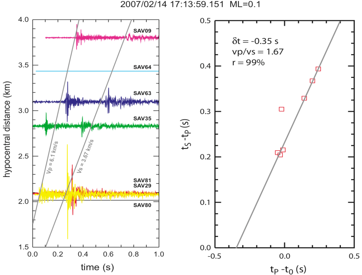
Figure 2. (left) Record section for a ML=0.1 event (vertical traces) at recorded at Savuka mine. Note that some traces (SAV64, SAV80) have a failed component and the time shift of trace SAV35. (right) Wadati diagram for the same event. Note how the point for SAV35 plots outside the Wadati line. The grey line is the LSQ fit to the points and has an associated V_p/V_s of 1.67, a correlation coefficient of 0.99, and a origin time correction of -0.35 s.
