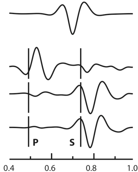
Figure 5. Impulse response for a 4.5 Hz instrument in the time-domain (top) and P-, SH-, and SV- recordings (bottom) of a mine-related event from station SAV29. Polarities can be assigned as negative (P), positive (SH), and positive (SH) after a visual comparison of the traces with the impulse response.
